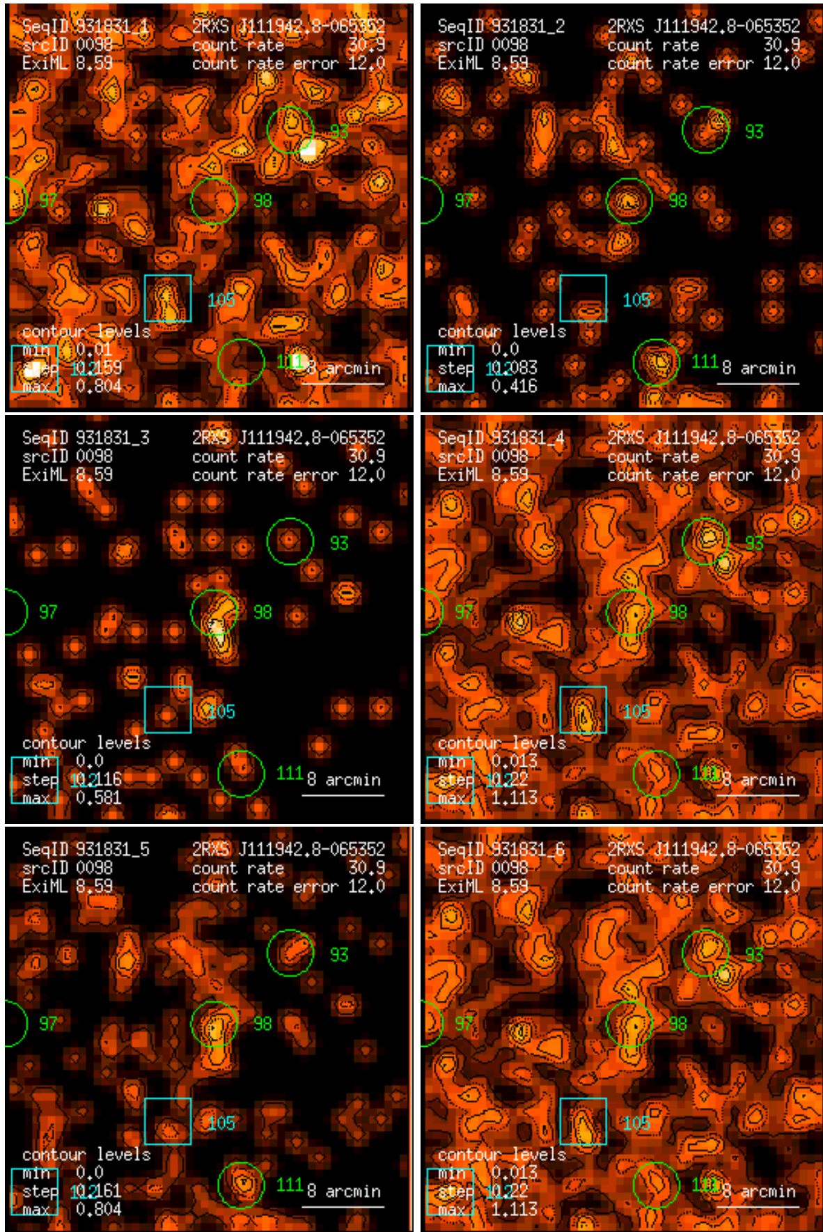
Figure 98: RASS 931831: detection 0098: band rate images, Gaussian filter: (1) PSPC channels 11 – 41, (2) 52 – 90, (3) 91 – 201, (4) 11 – 235, (5) 52 – 201, (6) 11 – 201. Broad band rates in counts/ks. Band rate contour levels in counts/ks/arcmin 2 .
