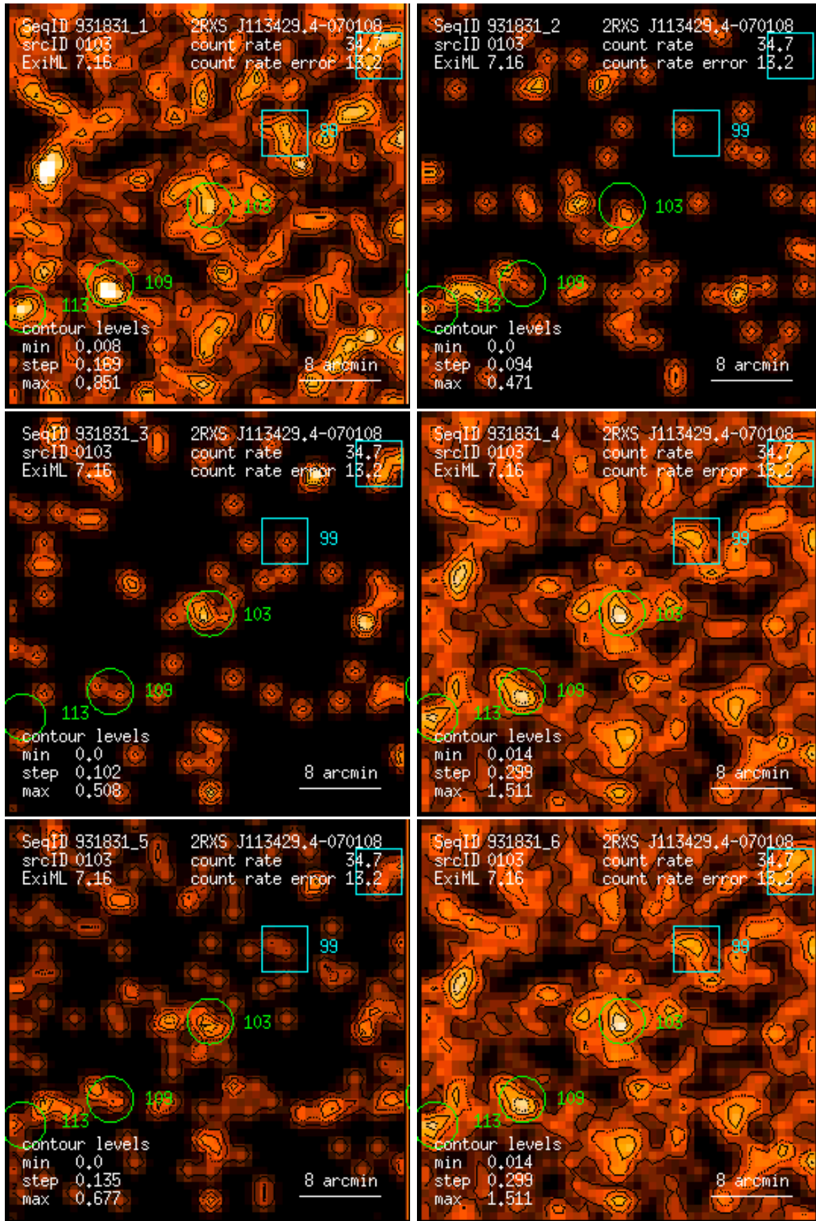
Figure 103: RASS 931831: detection 0103: band rate images, Gaussian filter: (1) PSPC channels 11 – 41, (2) 52 – 90, (3) 91 – 201, (4) 11 – 235, (5) 52 – 201, (6) 11 – 201. Broad band rates in counts/ks. Band rate contour levels in counts/ks/arcmin 2 .
