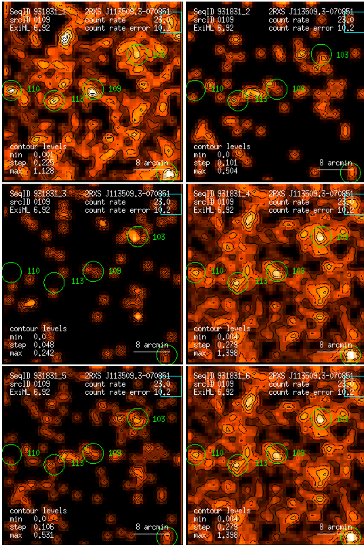
Figure 109: RASS 931831: detection 0109: band rate images, Gaussian filter: (1) PSPC channels 11 – 41, (2) 52 – 90, (3) 91 – 201, (4) 11 – 235, (5) 52 – 201, (6) 11 – 201. Broad band rates in counts/ks. Band rate contour levels in counts/ks/arcmin 2 .
