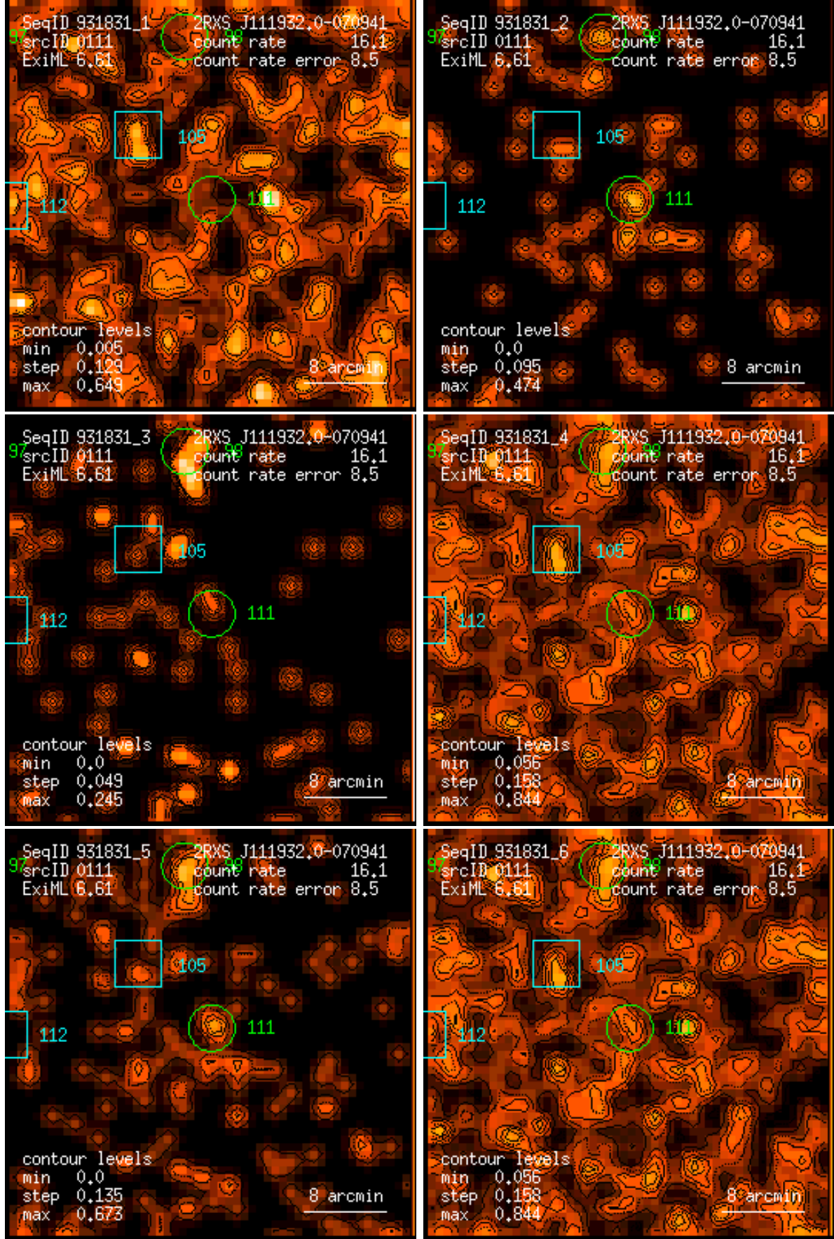
Figure 111: RASS 931831: detection 0111: band rate images, Gaussian filter: (1) PSPC channels 11 – 41, (2) 52 – 90, (3) 91 – 201, (4) 11 – 235, (5) 52 – 201, (6) 11 – 201. Broad band rates in counts/ks. Band rate contour levels in counts/ks/arcmin 2 .
