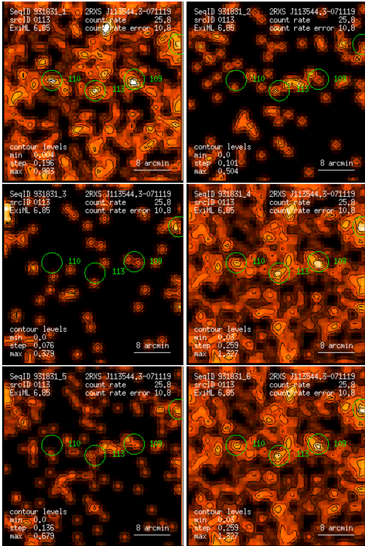
Figure 113: RASS 931831: detection 0113: band rate images, Gaussian filter: (1) PSPC channels 11 – 41, (2) 52 – 90, (3) 91 – 201, (4) 11 – 235, (5) 52 – 201, (6) 11 – 201. Broad band rates in counts/ks. Band rate contour levels in counts/ks/arcmin 2 .
