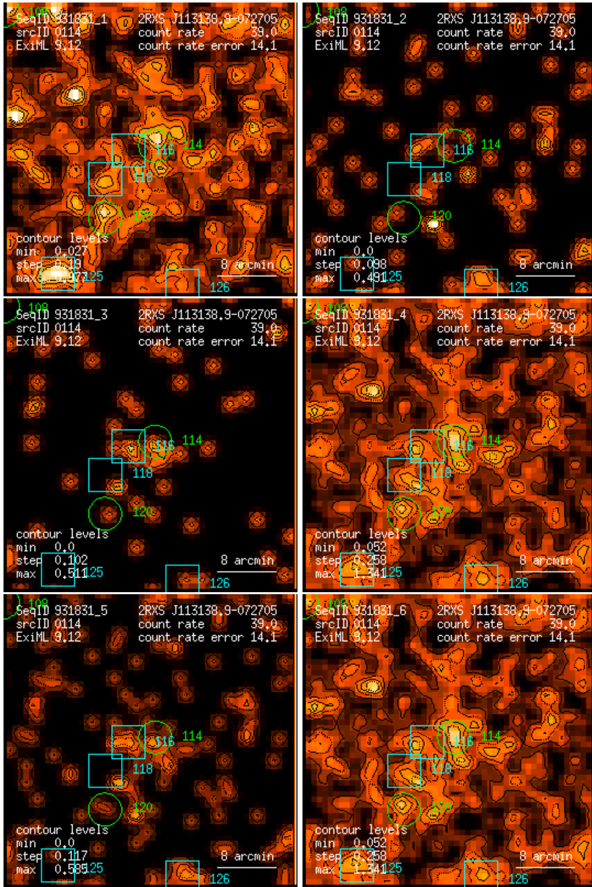
Figure 114: RASS 931831: detection 0114: band rate images, Gaussian filter: (1) PSPC channels 11 – 41, (2) 52 – 90, (3) 91 – 201, (4) 11 – 235, (5) 52 – 201, (6) 11 – 201. Broad band rates in counts/ks. Band rate contour levels in counts/ks/arcmin 2 .
