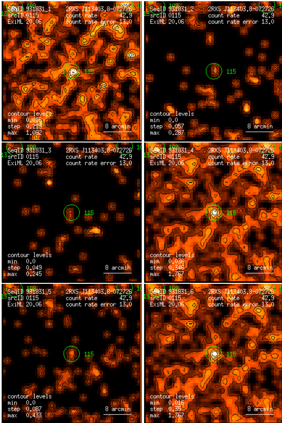
Figure 115: RASS 931831: detection 0115: band rate images, Gaussian filter: (1) PSPC channels 11 – 41, (2) 52 – 90, (3) 91 – 201, (4) 11 – 235, (5) 52 – 201, (6) 11 – 201. Broad band rates in counts/ks. Band rate contour levels in counts/ks/arcmin 2 .
