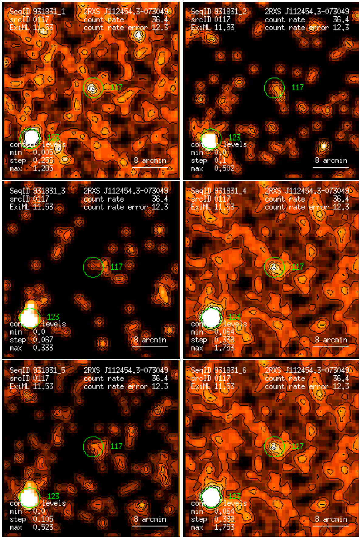
Figure 117: RASS 931831: detection 0117: band rate images, Gaussian filter: (1) PSPC channels 11 – 41, (2) 52 – 90, (3) 91 – 201, (4) 11 – 235, (5) 52 – 201, (6) 11 – 201. Broad band rates in counts/ks. Band rate contour levels in counts/ks/arcmin 2 .
