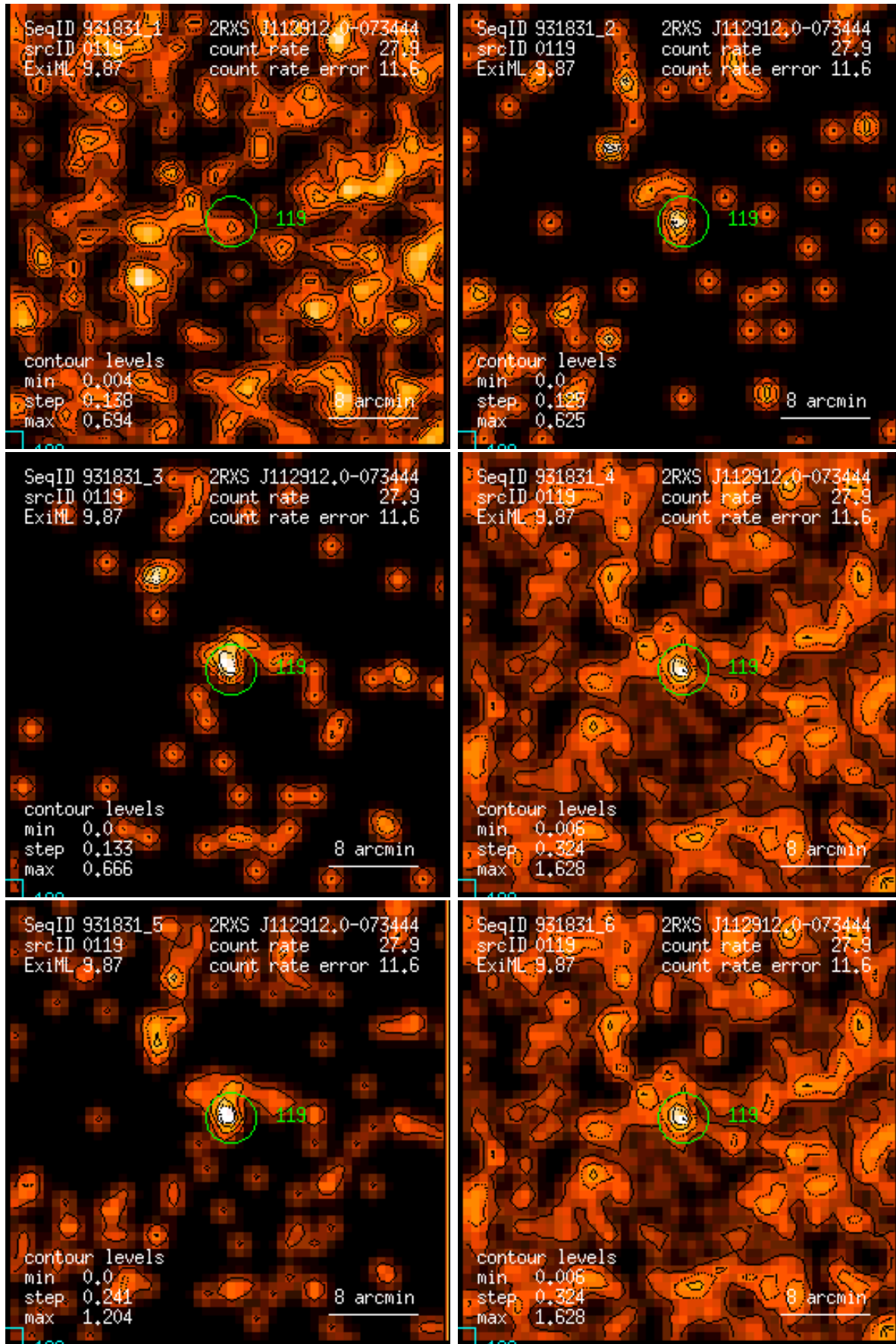
Figure 119: RASS 931831: detection 0119: band rate images, Gaussian filter: (1) PSPC channels 11 – 41, (2) 52 – 90, (3) 91 – 201, (4) 11 – 235, (5) 52 – 201, (6) 11 – 201. Broad band rates in counts/ks. Band rate contour levels in counts/ks/arcmin 2 .
