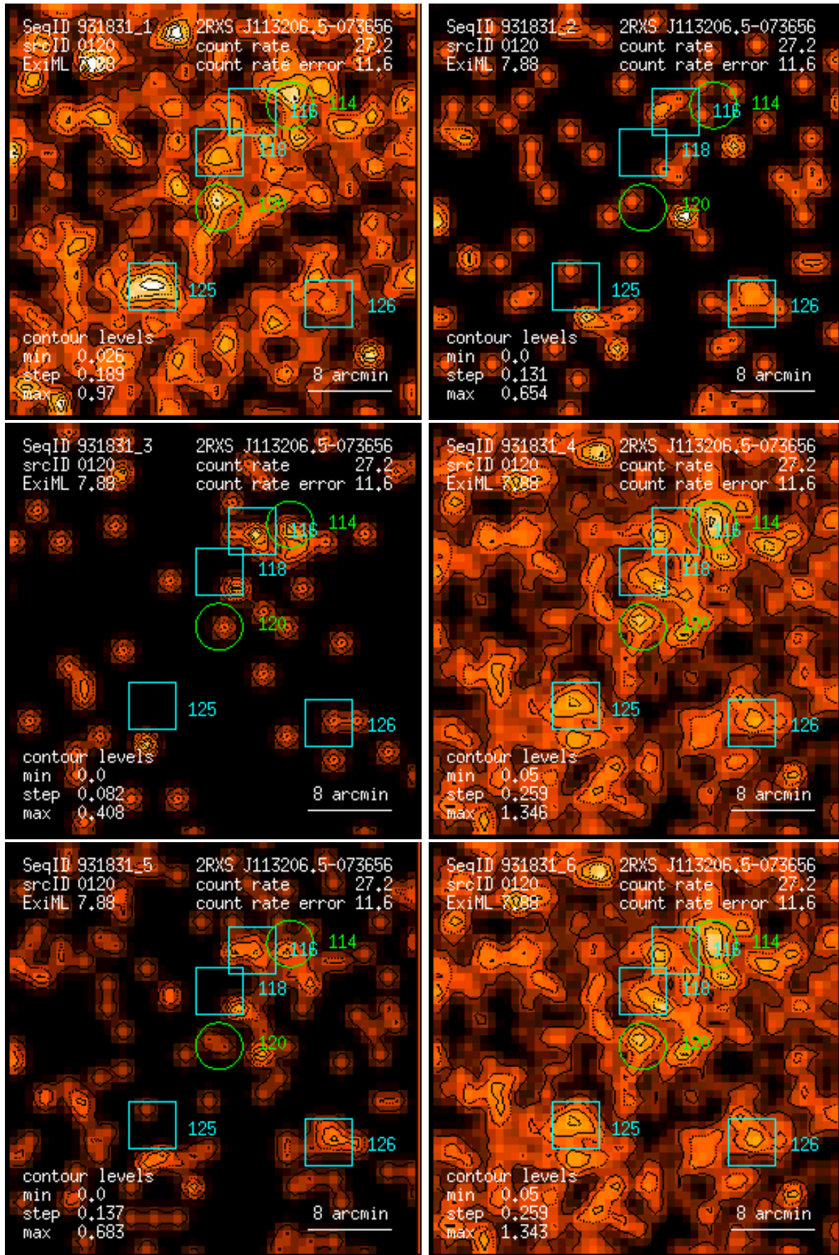
Figure 120: RASS 931831: detection 0120: band rate images, Gaussian filter: (1) PSPC channels 11 – 41, (2) 52 – 90, (3) 91 – 201, (4) 11 – 235, (5) 52 – 201, (6) 11 – 201. Broad band rates in counts/ks. Band rate contour levels in counts/ks/arcmin 2 .
