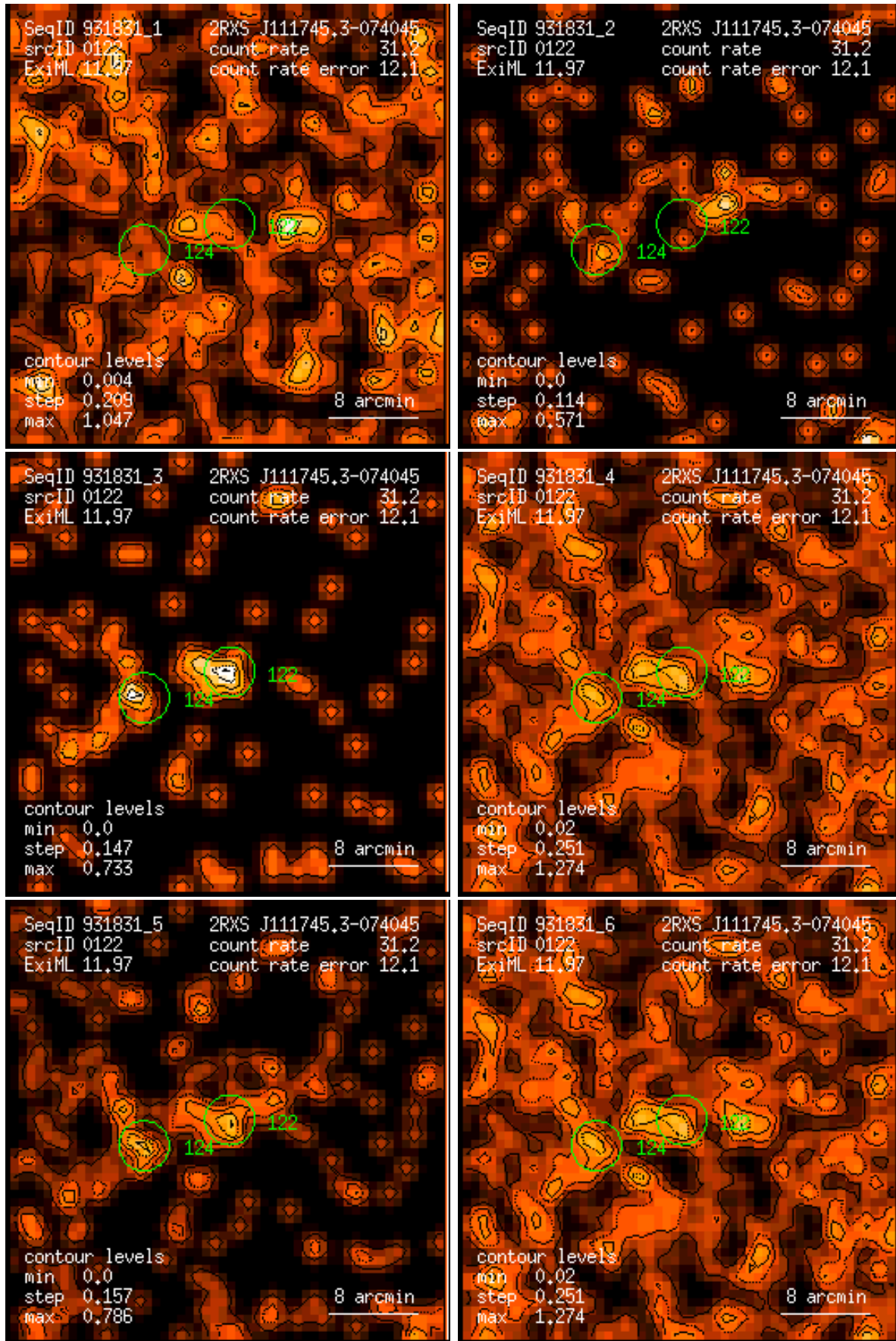
Figure 122: RASS 931831: detection 0122: band rate images, Gaussian filter: (1) PSPC channels 11 – 41, (2) 52 – 90, (3) 91 – 201, (4) 11 – 235, (5) 52 – 201, (6) 11 – 201. Broad band rates in counts/ks. Band rate contour levels in counts/ks/arcmin 2 .
