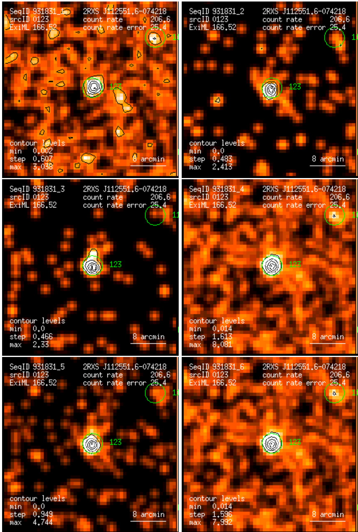
Figure 123: RASS 931831: detection 0123: band rate images, Gaussian filter: (1) PSPC channels 11 – 41, (2) 52 – 90, (3) 91 – 201, (4) 11 – 235, (5) 52 – 201, (6) 11 – 201. Broad band rates in counts/ks. Band rate contour levels in counts/ks/arcmin 2 .
