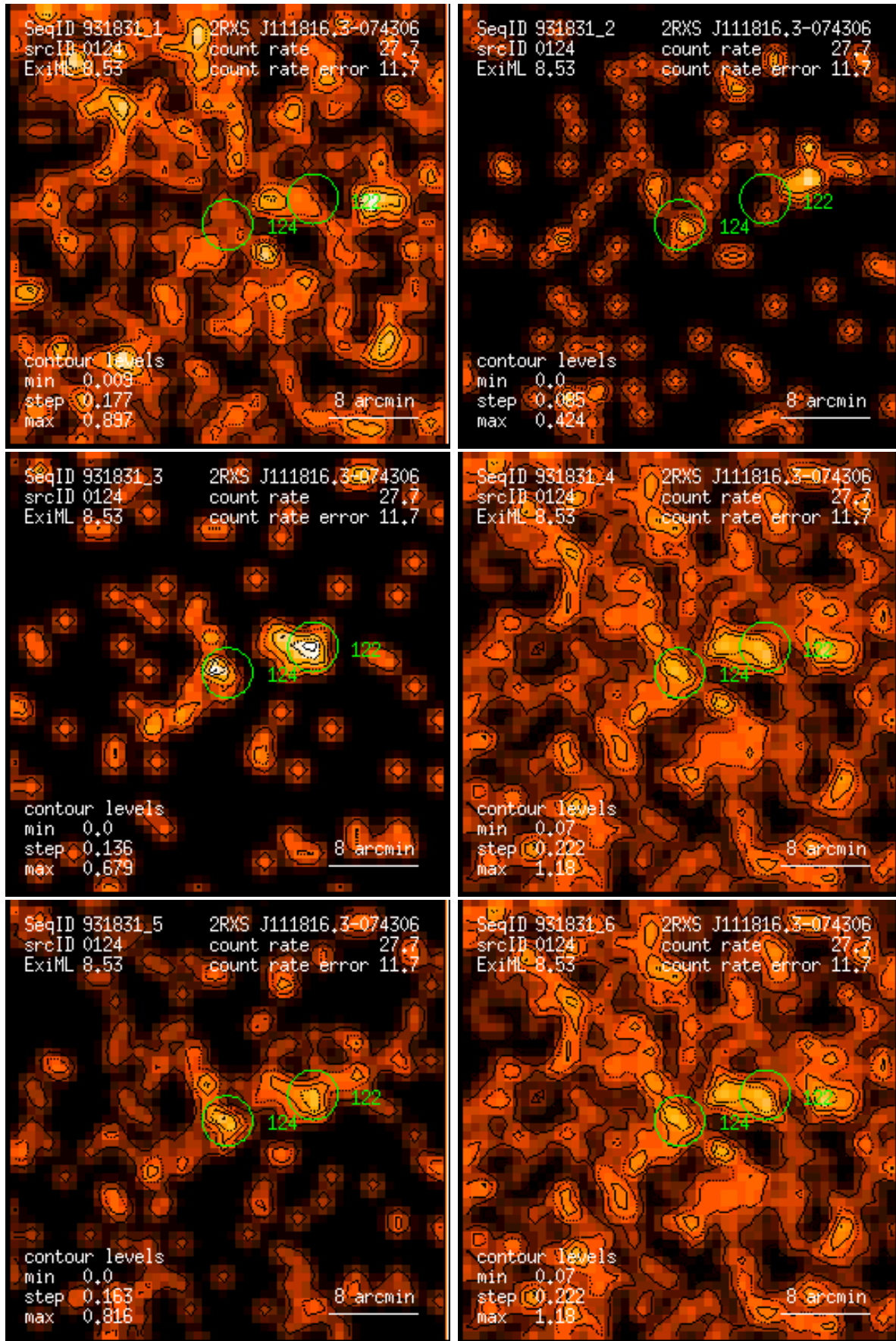
Figure 124: RASS 931831: detection 0124: band rate images, Gaussian filter: (1) PSPC channels 11 – 41, (2) 52 – 90, (3) 91 – 201, (4) 11 – 235, (5) 52 – 201, (6) 11 – 201. Broad band rates in counts/ks. Band rate contour levels in counts/ks/arcmin 2 .
