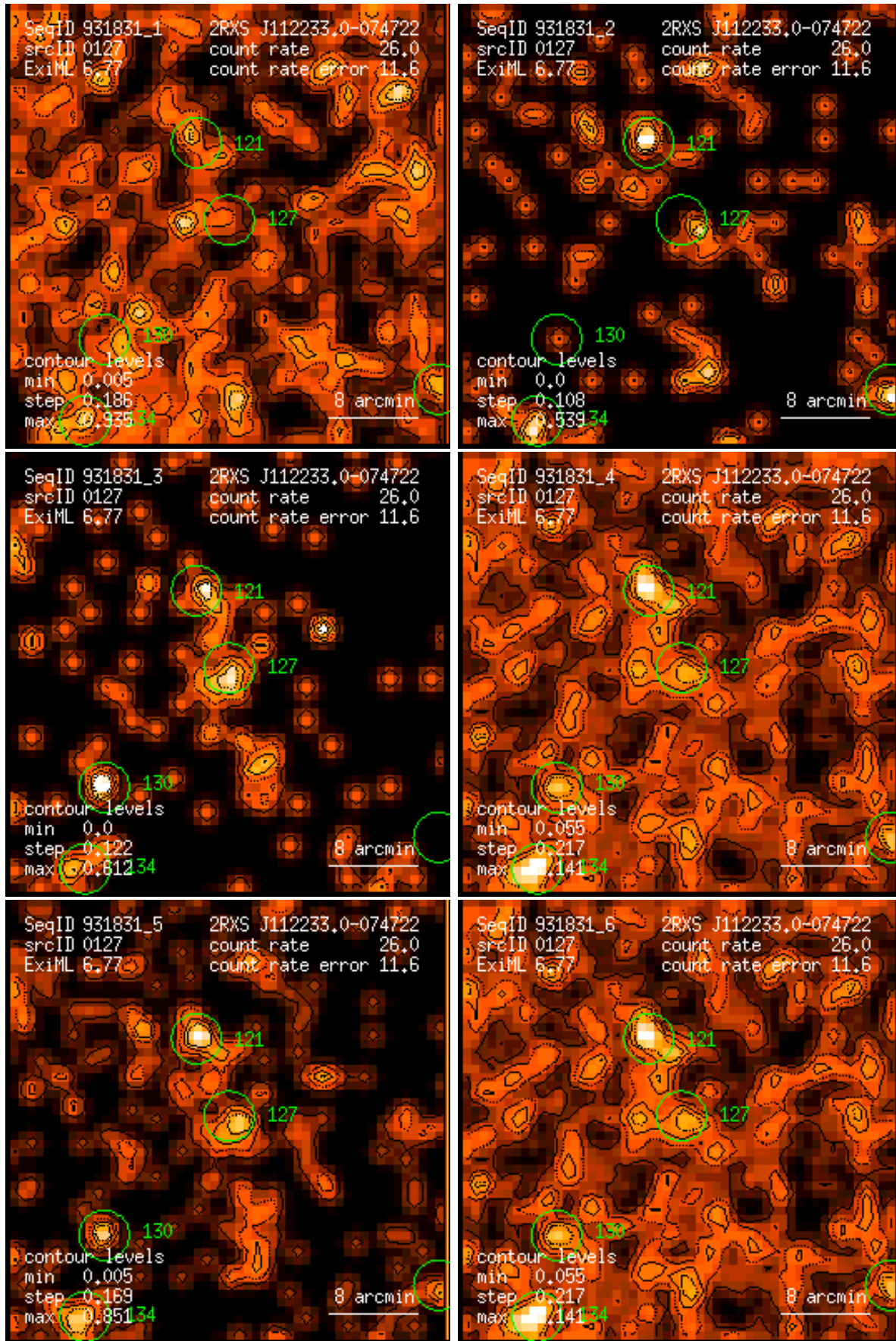
Figure 127: RASS 931831: detection 0127: band rate images, Gaussian filter: (1) PSPC channels 11 – 41, (2) 52 – 90, (3) 91 – 201, (4) 11 – 235, (5) 52 – 201, (6) 11 – 201. Broad band rates in counts/ks. Band rate contour levels in counts/ks/arcmin 2 .
