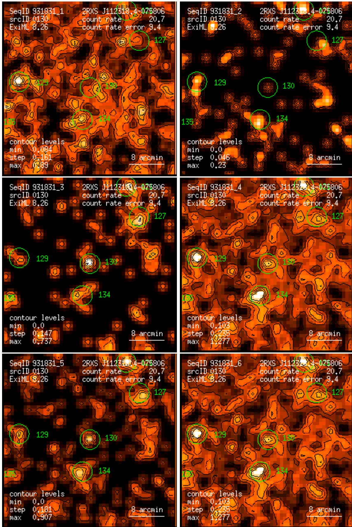
Figure 130: RASS 931831: detection 0130: band rate images, Gaussian filter: (1) PSPC channels 11 – 41, (2) 52 – 90, (3) 91 – 201, (4) 11 – 235, (5) 52 – 201, (6) 11 – 201. Broad band rates in counts/ks. Band rate contour levels in counts/ks/arcmin 2 .
