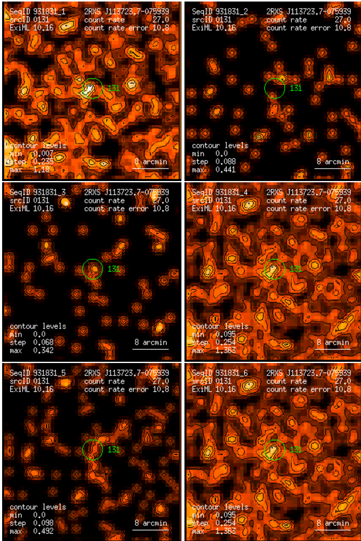
Figure 131: RASS 931831: detection 0131: band rate images, Gaussian filter: (1) PSPC channels 11 – 41, (2) 52 – 90, (3) 91 – 201, (4) 11 – 235, (5) 52 – 201, (6) 11 – 201. Broad band rates in counts/ks. Band rate contour levels in counts/ks/arcmin 2 .
