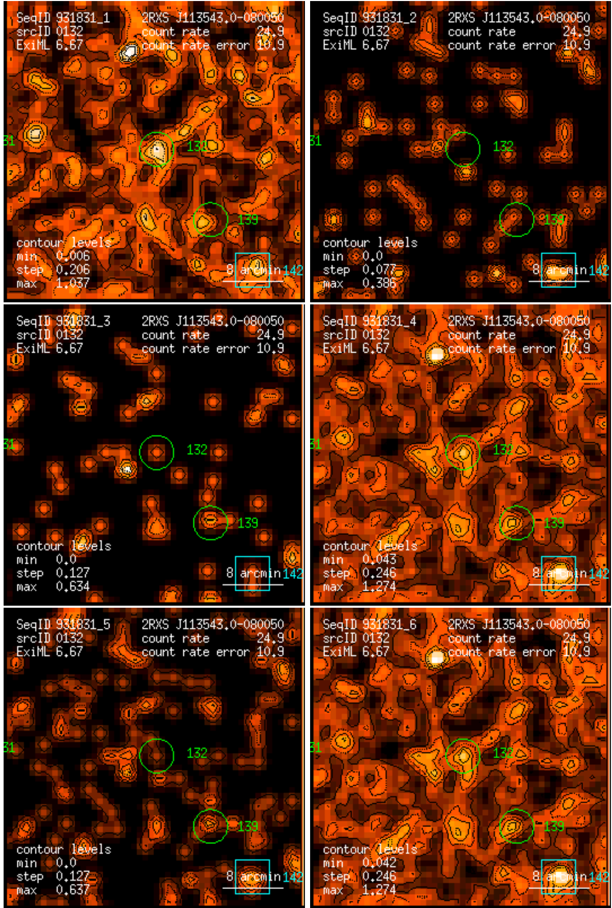
Figure 132: RASS 931831: detection 0132: band rate images, Gaussian filter: (1) PSPC channels 11 – 41, (2) 52 – 90, (3) 91 – 201, (4) 11 – 235, (5) 52 – 201, (6) 11 – 201. Broad band rates in counts/ks. Band rate contour levels in counts/ks/arcmin 2 .
