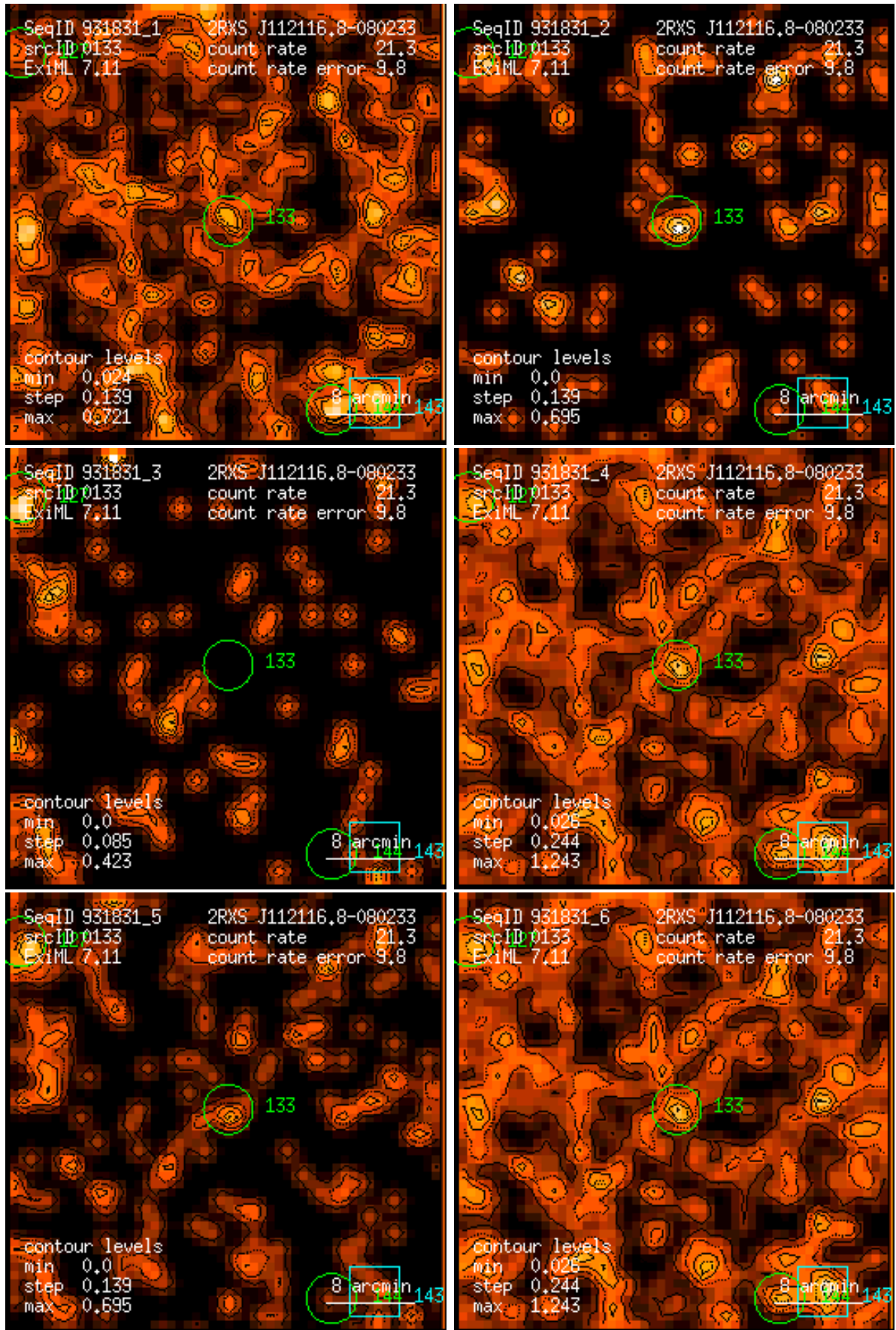
Figure 133: RASS 931831: detection 0133: band rate images, Gaussian filter: (1) PSPC channels 11 – 41, (2) 52 – 90, (3) 91 – 201, (4) 11 – 235, (5) 52 – 201, (6) 11 – 201. Broad band rates in counts/ks. Band rate contour levels in counts/ks/arcmin 2 .
