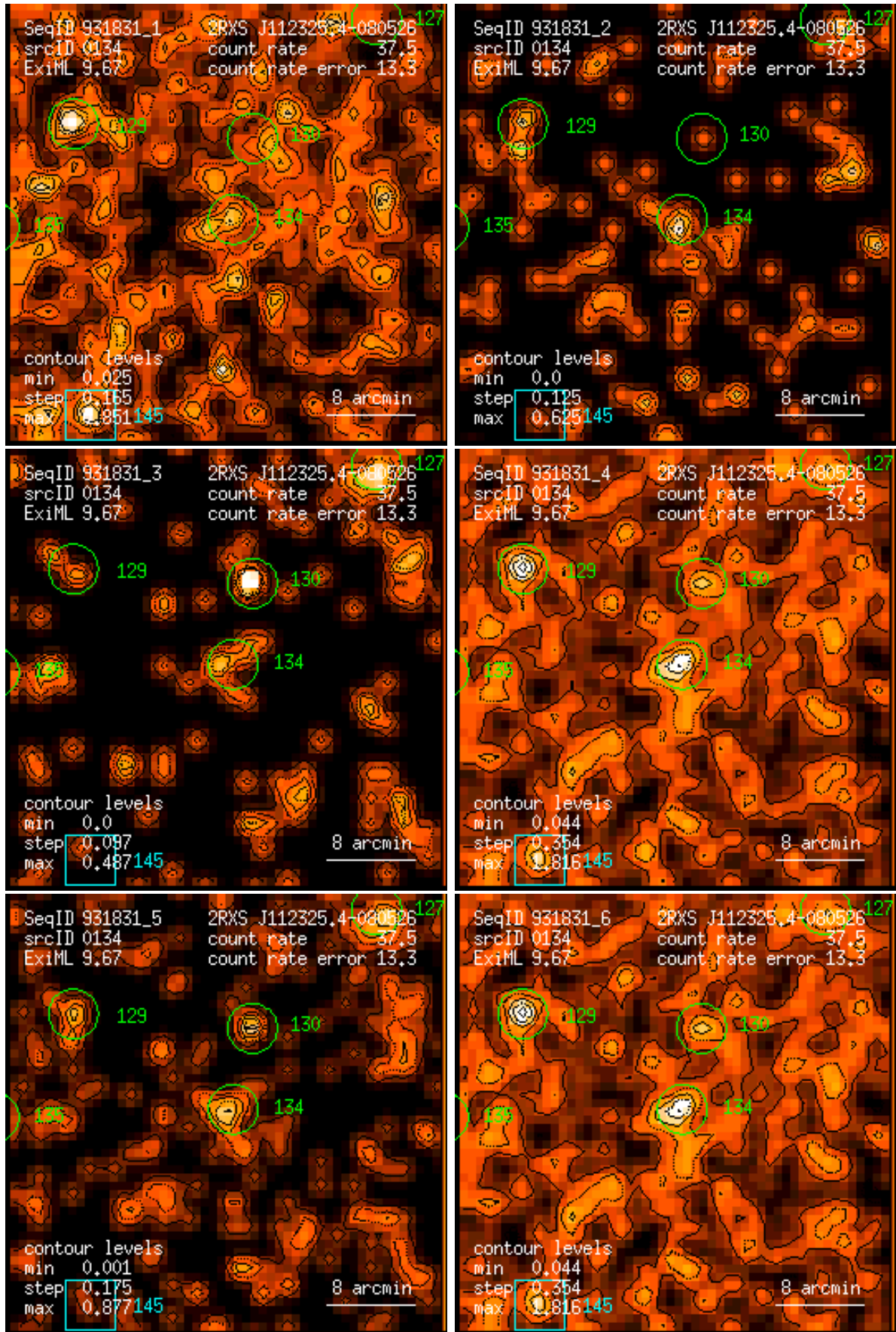
Figure 134: RASS 931831: detection 0134: band rate images, Gaussian filter: (1) PSPC channels 11 – 41, (2) 52 – 90, (3) 91 – 201, (4) 11 – 235, (5) 52 – 201, (6) 11 – 201. Broad band rates in counts/ks. Band rate contour levels in counts/ks/arcmin 2 .
