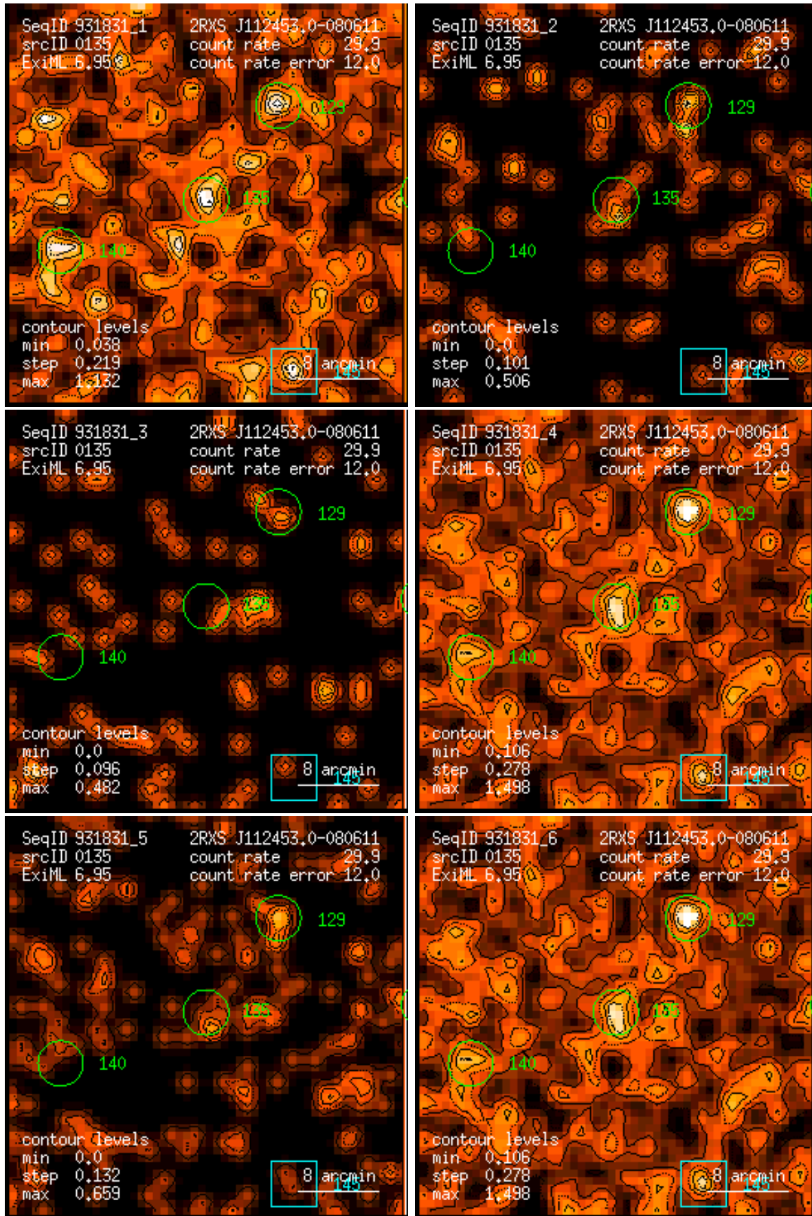
Figure 135: RASS 931831: detection 0135: band rate images, Gaussian filter: (1) PSPC channels 11 – 41, (2) 52 – 90, (3) 91 – 201, (4) 11 – 235, (5) 52 – 201, (6) 11 – 201. Broad band rates in counts/ks. Band rate contour levels in counts/ks/arcmin 2 .
