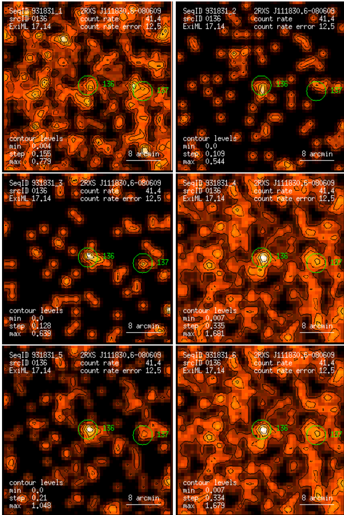
Figure 136: RASS 931831: detection 0136: band rate images, Gaussian filter: (1) PSPC channels 11 – 41, (2) 52 – 90, (3) 91 – 201, (4) 11 – 235, (5) 52 – 201, (6) 11 – 201. Broad band rates in counts/ks. Band rate contour levels in counts/ks/arcmin 2 .
