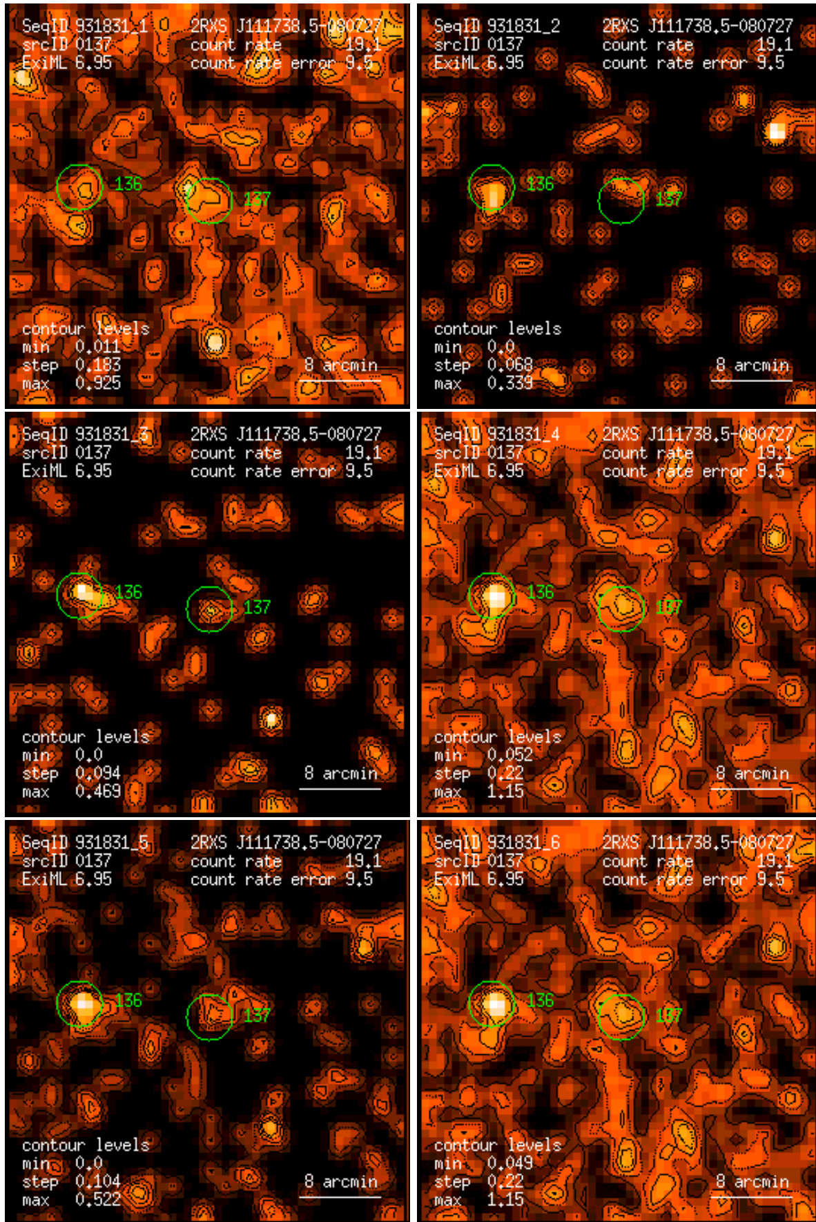
Figure 137: RASS 931831: detection 0137: band rate images, Gaussian filter: (1) PSPC channels 11 – 41, (2) 52 – 90, (3) 91 – 201, (4) 11 – 235, (5) 52 – 201, (6) 11 – 201. Broad band rates in counts/ks. Band rate contour levels in counts/ks/arcmin 2 .
