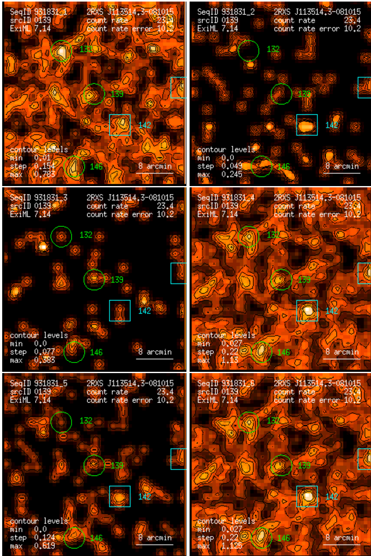
Figure 139: RASS 931831: detection 0139: band rate images, Gaussian filter: (1) PSPC channels 11 – 41, (2) 52 – 90, (3) 91 – 201, (4) 11 – 235, (5) 52 – 201, (6) 11 – 201. Broad band rates in counts/ks. Band rate contour levels in counts/ks/arcmin 2 .
