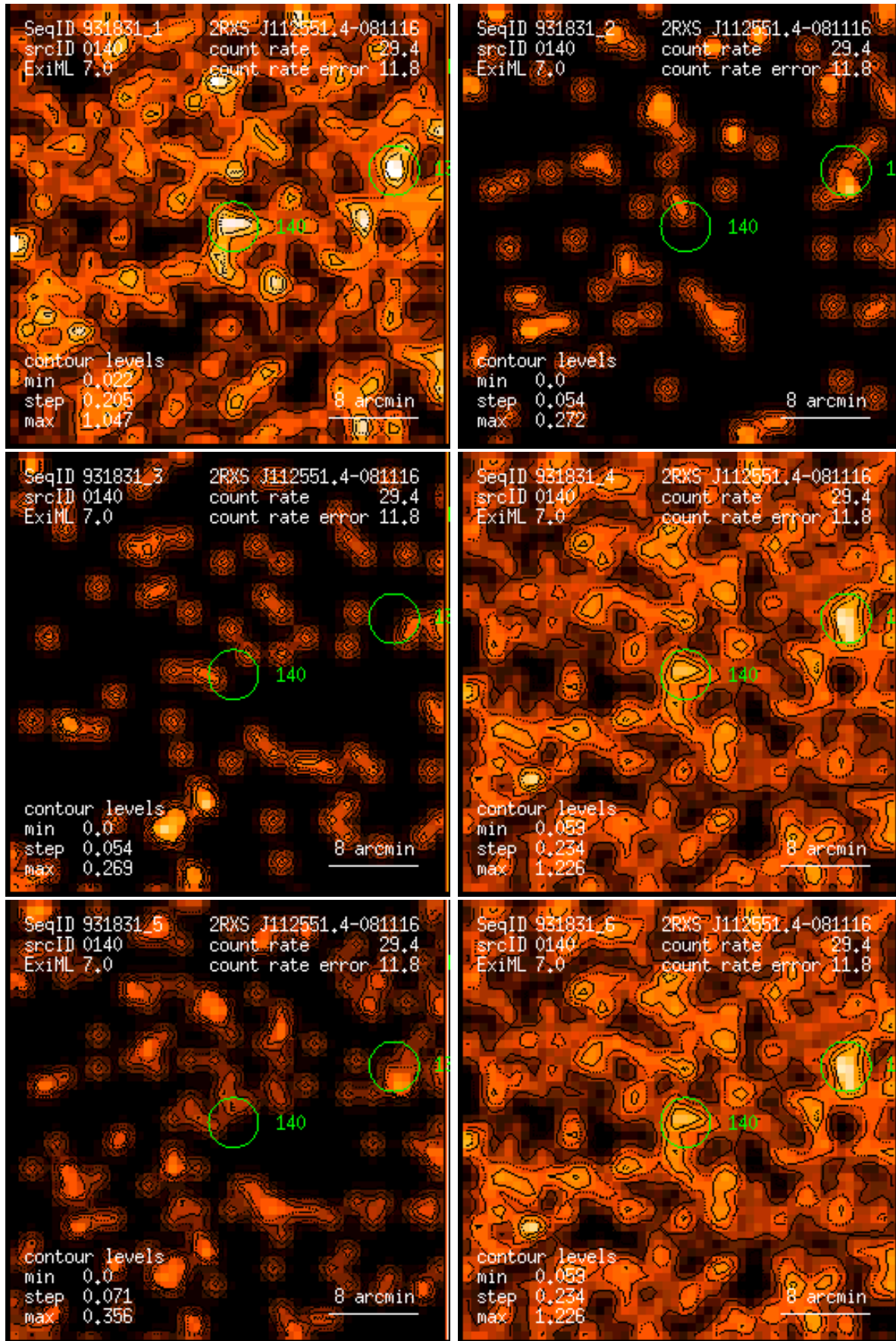
Figure 140: RASS 931831: detection 0140: band rate images, Gaussian filter: (1) PSPC channels 11 – 41, (2) 52 – 90, (3) 91 – 201, (4) 11 – 235, (5) 52 – 201, (6) 11 – 201. Broad band rates in counts/ks. Band rate contour levels in counts/ks/arcmin 2 .
