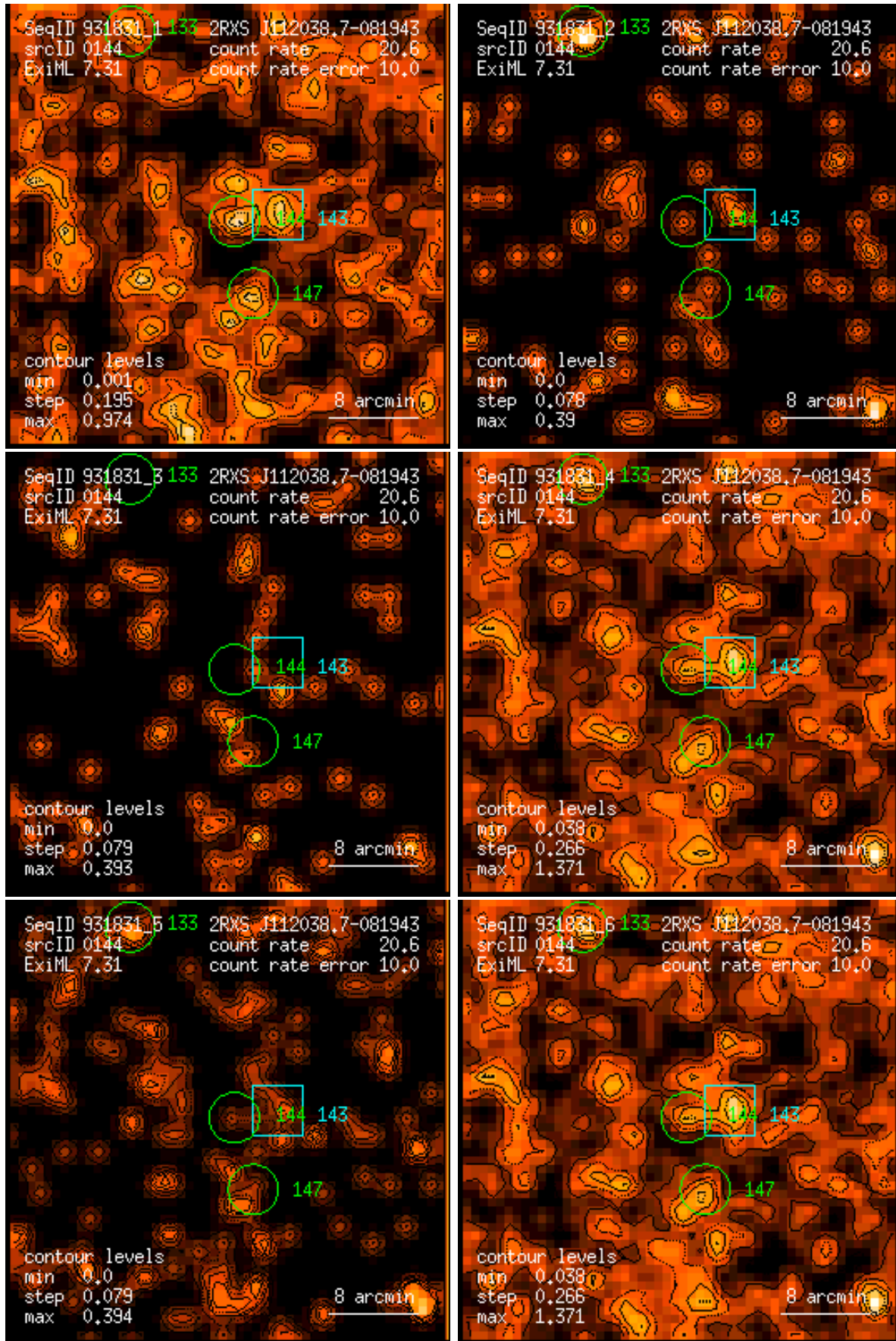
Figure 144: RASS 931831: detection 0144: band rate images, Gaussian filter: (1) PSPC channels 11 – 41, (2) 52 – 90, (3) 91 – 201, (4) 11 – 235, (5) 52 – 201, (6) 11 – 201. Broad band rates in counts/ks. Band rate contour levels in counts/ks/arcmin 2 .
