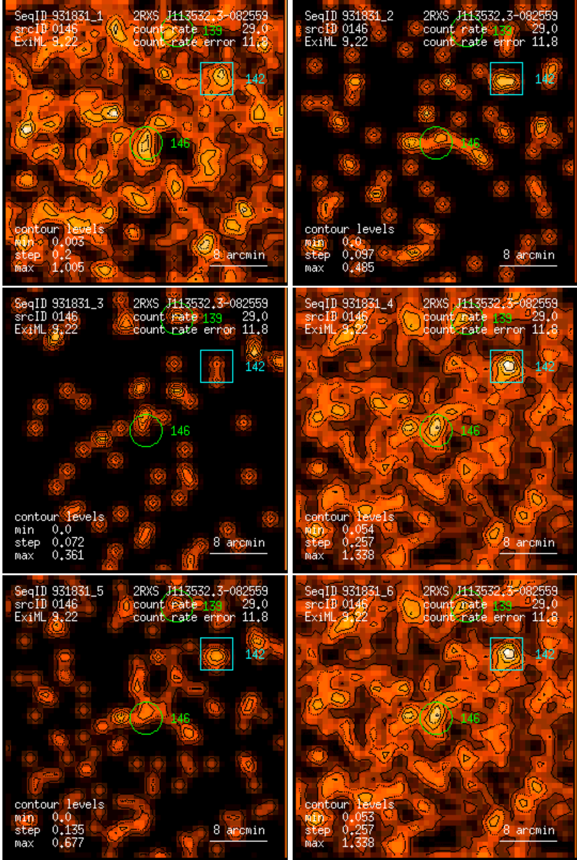
Figure 146: RASS 931831: detection 0146: band rate images, Gaussian filter: (1) PSPC channels 11 – 41, (2) 52 – 90, (3) 91 – 201, (4) 11 – 235, (5) 52 – 201, (6) 11 – 201. Broad band rates in counts/ks. Band rate contour levels in counts/ks/arcmin 2 .
