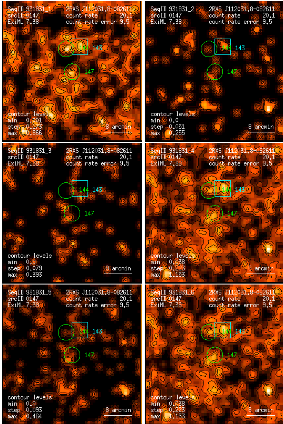
Figure 147: RASS 931831: detection 0147: band rate images, Gaussian filter: (1) PSPC channels 11 – 41, (2) 52 – 90, (3) 91 – 201, (4) 11 – 235, (5) 52 – 201, (6) 11 – 201. Broad band rates in counts/ks. Band rate contour levels in counts/ks/arcmin 2 .
