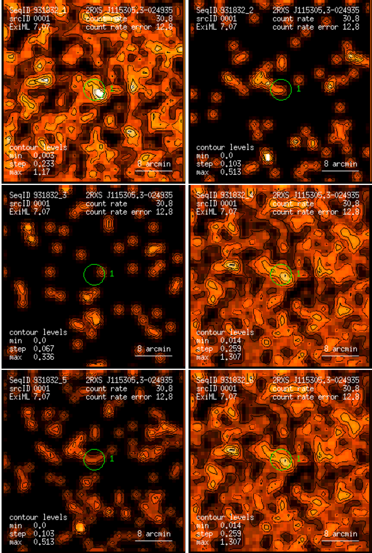
Figure 1: RASS 931832: detection 0001: band rate images, Gaussian filter: (1) PSPC channels 11 – 41, (2) 52 – 90, (3) 91 – 201, (4) 11 – 235, (5) 52 – 201, (6) 11 – 201. Broad band rates in counts/ks. Band rate contour levels in counts/ks/arcmin 2 .
