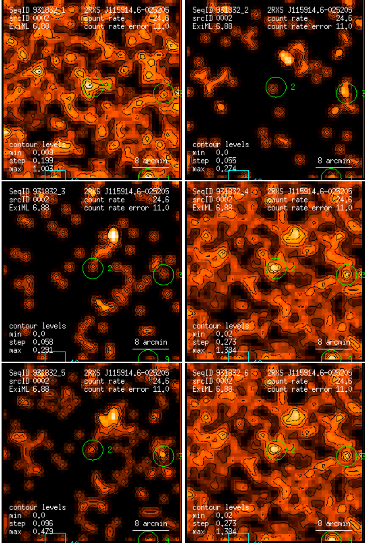
Figure 2: RASS 931832: detection 0002: band rate images, Gaussian filter: (1) PSPC channels 11 – 41, (2) 52 – 90, (3) 91 – 201, (4) 11 – 235, (5) 52 – 201, (6) 11 – 201. Broad band rates in counts/ks. Band rate contour levels in counts/ks/arcmin 2 .
