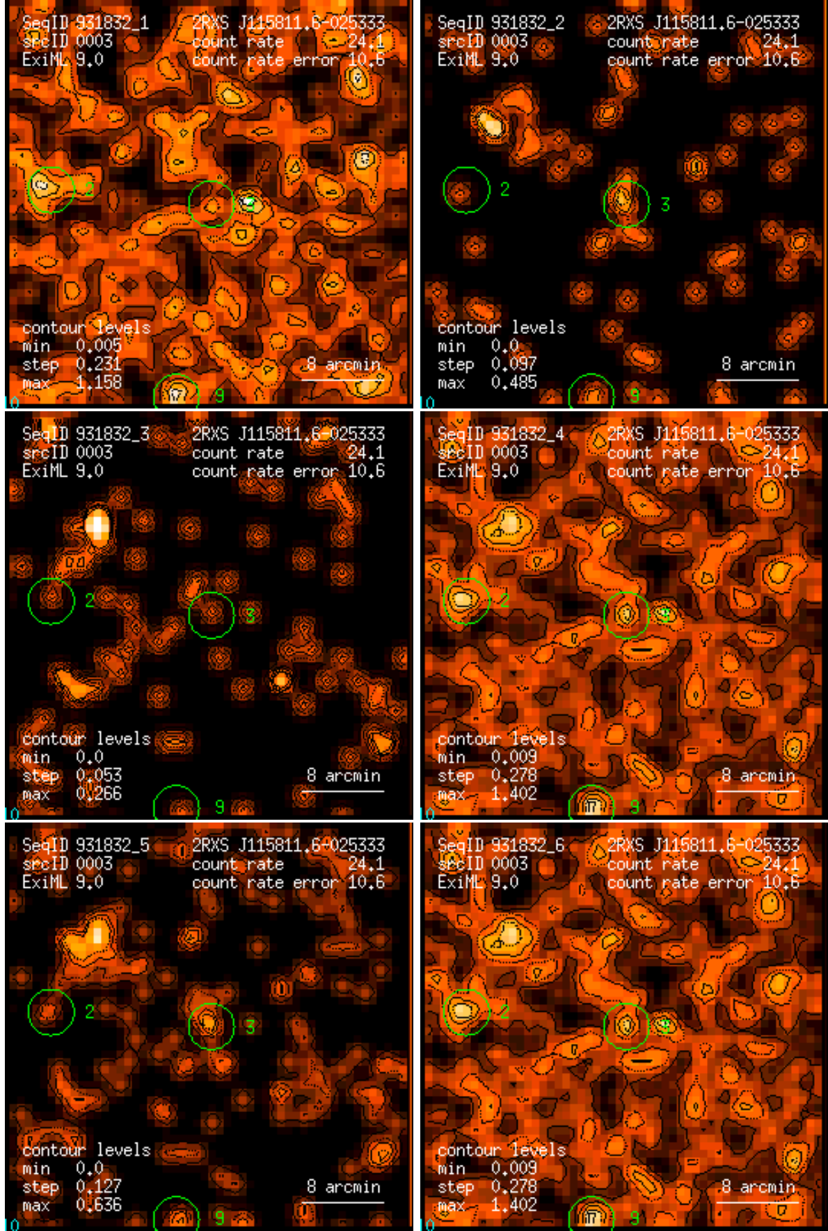
Figure 3: RASS 931832: detection 0003: band rate images, Gaussian filter: (1) PSPC channels 11 – 41, (2) 52 – 90, (3) 91 – 201, (4) 11 – 235, (5) 52 – 201, (6) 11 – 201. Broad band rates in counts/ks. Band rate contour levels in counts/ks/arcmin 2 .
