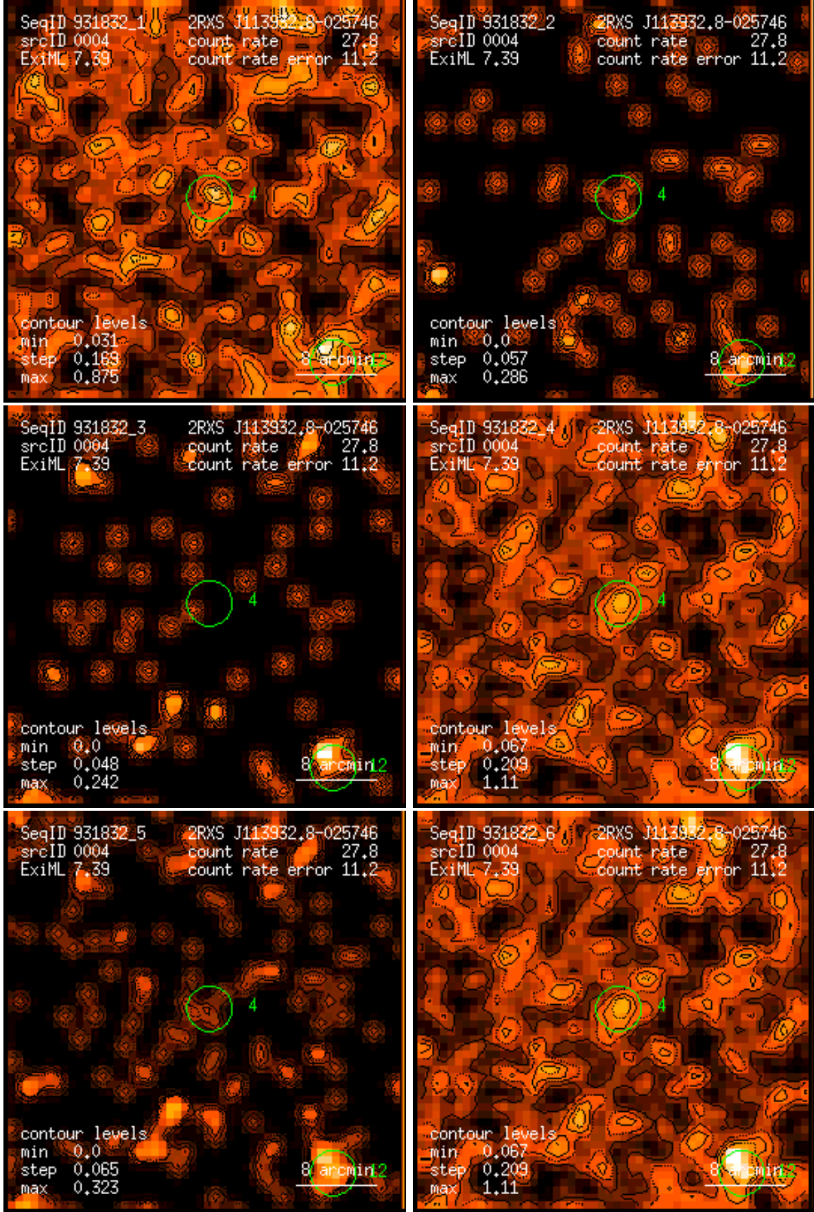
Figure 4: RASS 931832: detection 0004: band rate images, Gaussian filter: (1) PSPC channels 11 – 41, (2) 52 – 90, (3) 91 – 201, (4) 11 – 235, (5) 52 – 201, (6) 11 – 201. Broad band rates in counts/ks. Band rate contour levels in counts/ks/arcmin 2 .
