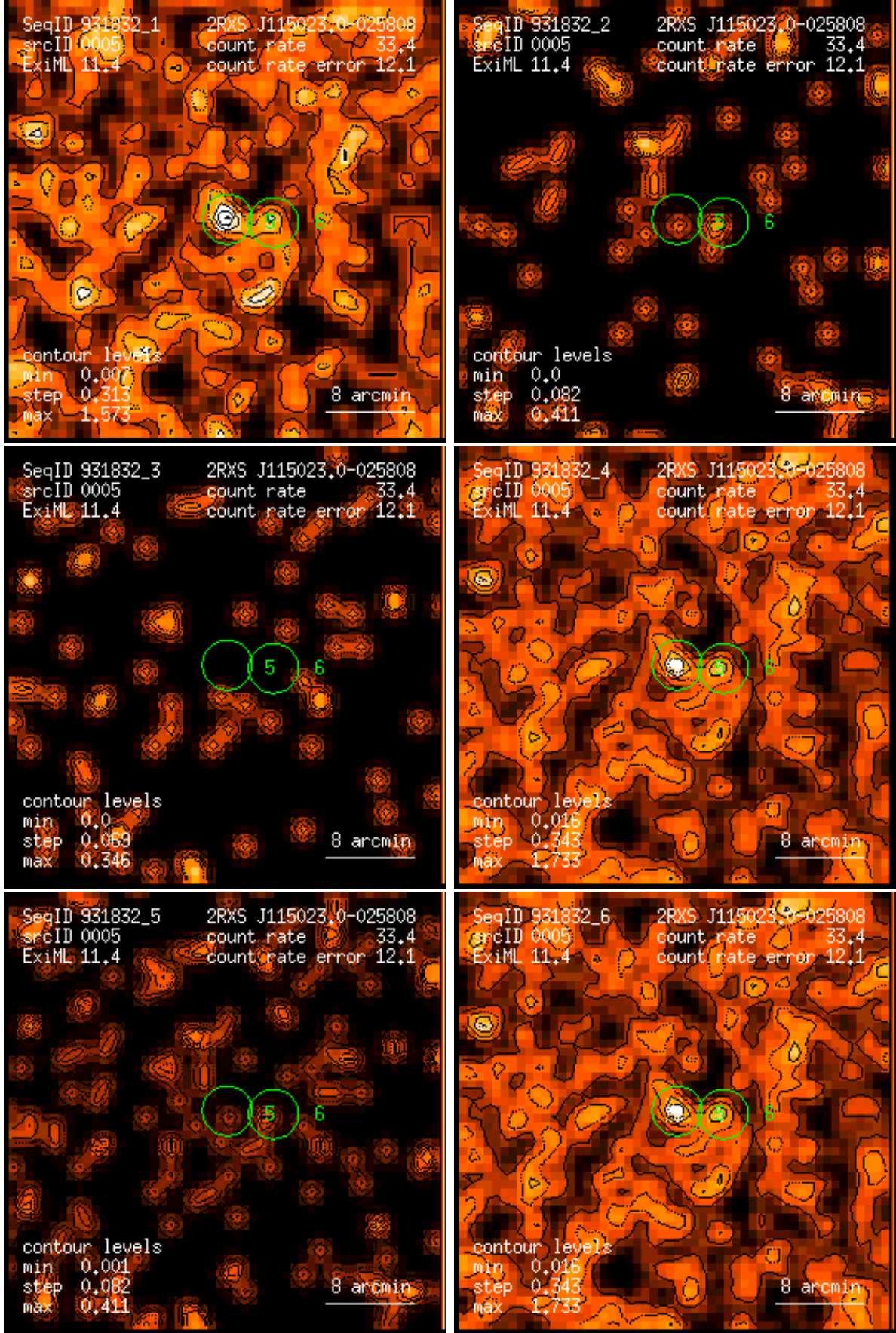
Figure 5: RASS 931832: detection 0005: band rate images, Gaussian filter: (1) PSPC channels 11 – 41, (2) 52 – 90, (3) 91 – 201, (4) 11 – 235, (5) 52 – 201, (6) 11 – 201. Broad band rates in counts/ks. Band rate contour levels in counts/ks/arcmin 2 .
