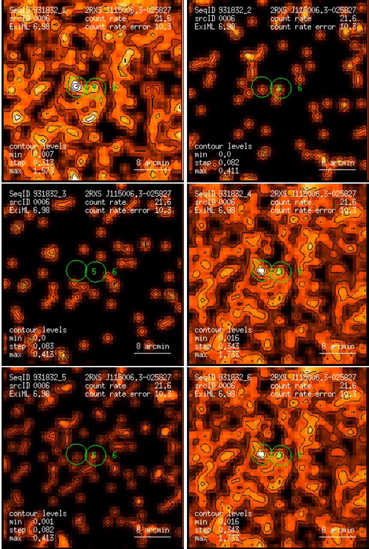
Figure 6: RASS 931832: detection 0006: band rate images, Gaussian filter: (1) PSPC channels 11 – 41, (2) 52 – 90, (3) 91 – 201, (4) 11 – 235, (5) 52 – 201, (6) 11 – 201. Broad band rates in counts/ks. Band rate contour levels in counts/ks/arcmin 2 .
