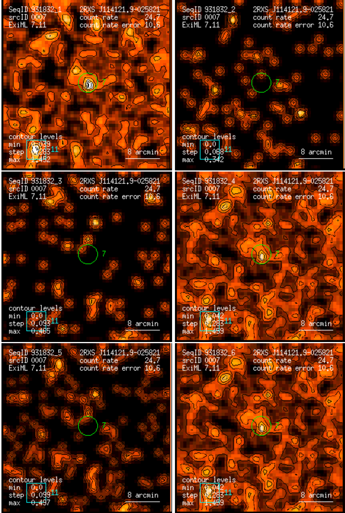
Figure 7: RASS 931832: detection 0007: band rate images, Gaussian filter: (1) PSPC channels 11 – 41, (2) 52 – 90, (3) 91 – 201, (4) 11 – 235, (5) 52 – 201, (6) 11 – 201. Broad band rates in counts/ks. Band rate contour levels in counts/ks/arcmin 2 .
