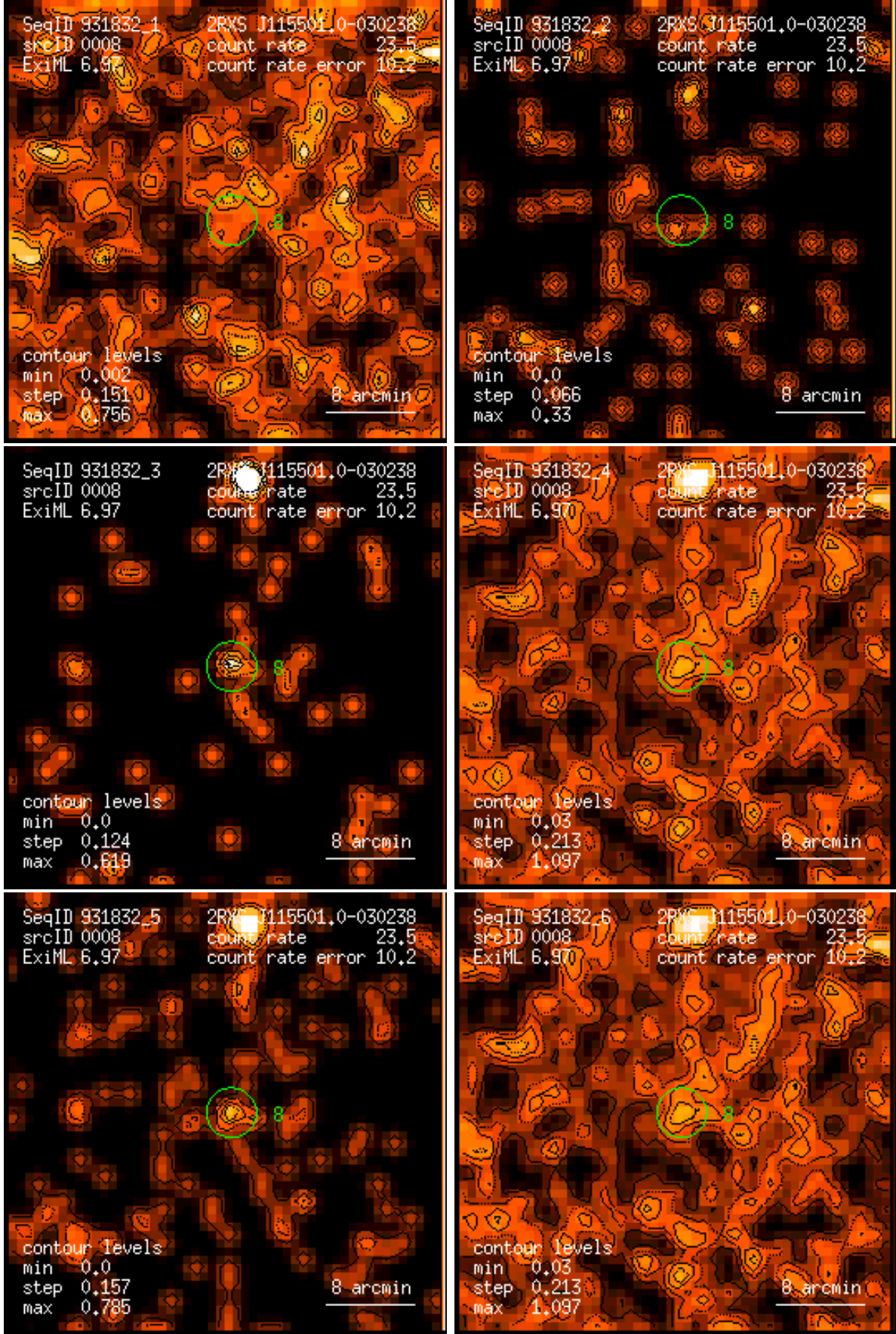
Figure 8: RASS 931832: detection 0008: band rate images, Gaussian filter: (1) PSPC channels 11 – 41, (2) 52 – 90, (3) 91 – 201, (4) 11 – 235, (5) 52 – 201, (6) 11 – 201. Broad band rates in counts/ks. Band rate contour levels in counts/ks/arcmin 2 .
