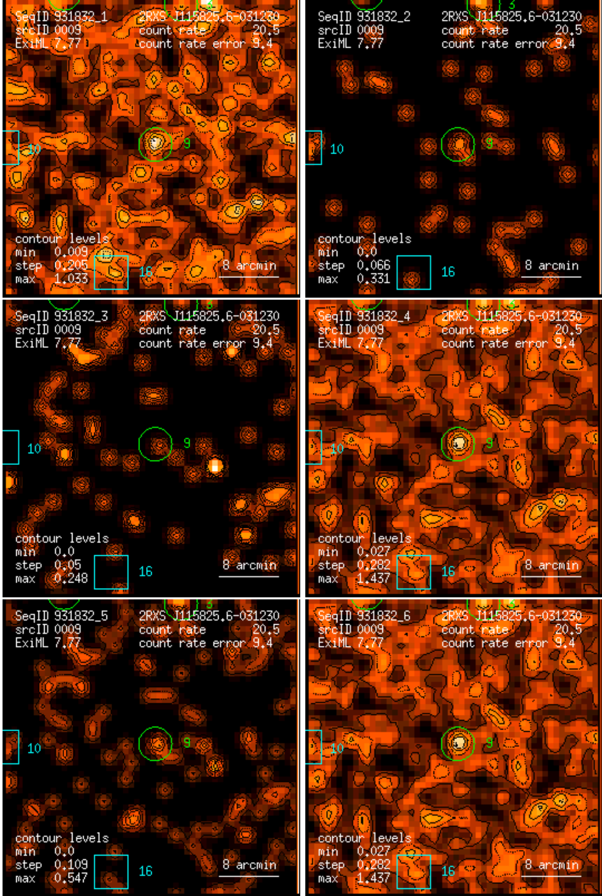
Figure 9: RASS 931832: detection 0009: band rate images, Gaussian filter: (1) PSPC channels 11 – 41, (2) 52 – 90, (3) 91 – 201, (4) 11 – 235, (5) 52 – 201, (6) 11 – 201. Broad band rates in counts/ks. Band rate contour levels in counts/ks/arcmin 2 .
