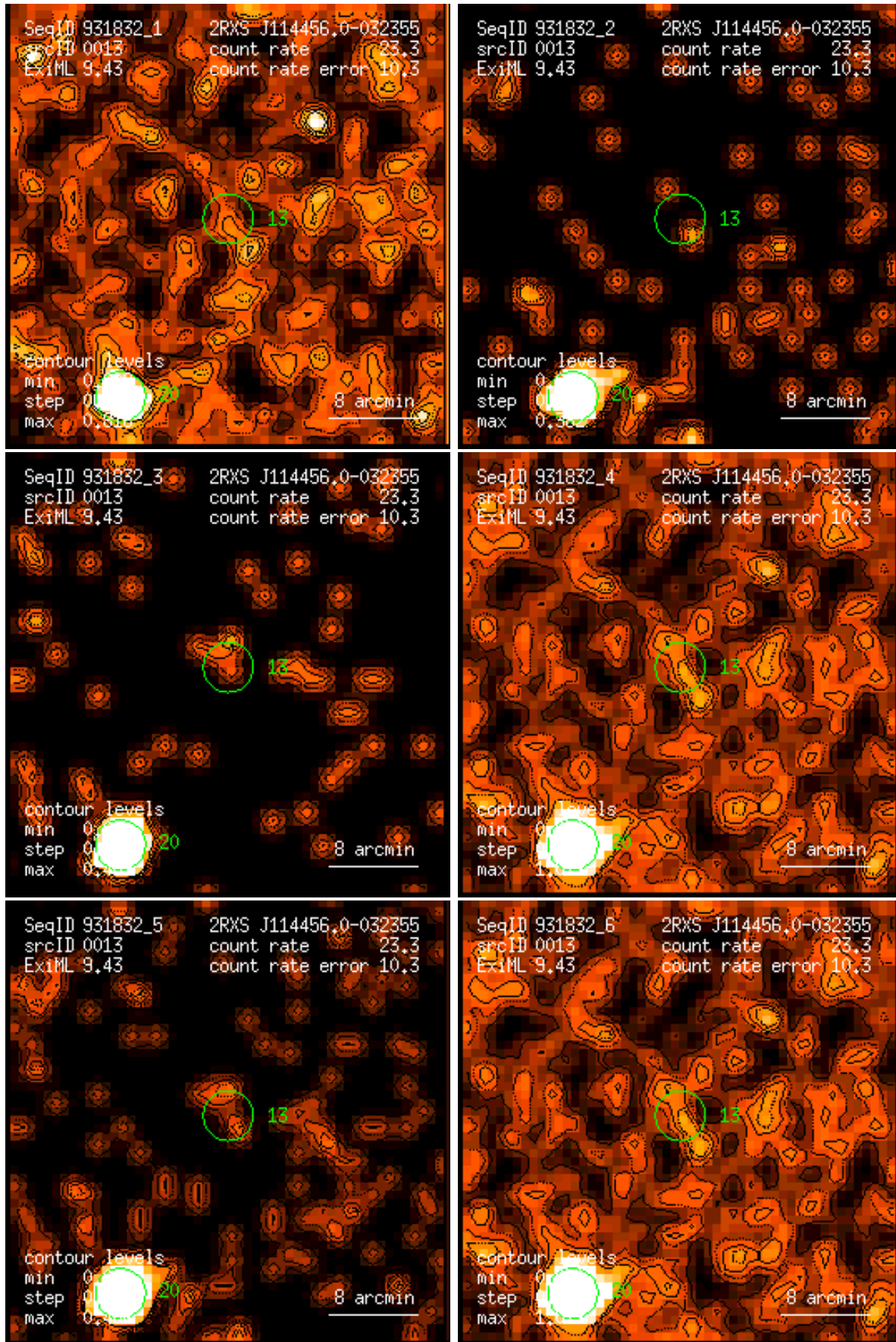
Figure 13: RASS 931832: detection 0013: band rate images, Gaussian filter: (1) PSPC channels 11 – 41, (2) 52 – 90, (3) 91 – 201, (4) 11 – 235, (5) 52 – 201, (6) 11 – 201. Broad band rates in counts/ks. Band rate contour levels in counts/ks/arcmin 2 .
