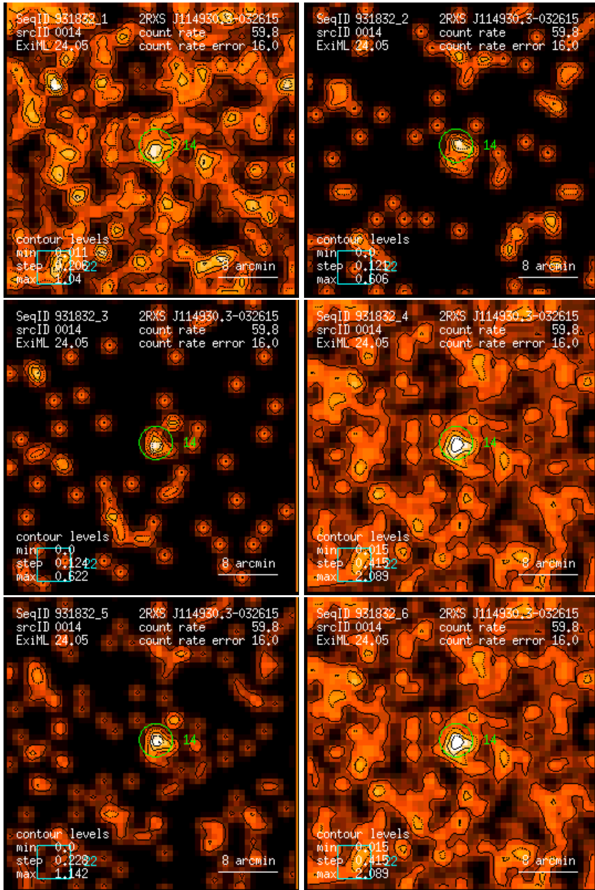
Figure 14: RASS 931832: detection 0014: band rate images, Gaussian filter: (1) PSPC channels 11 – 41, (2) 52 – 90, (3) 91 – 201, (4) 11 – 235, (5) 52 – 201, (6) 11 – 201. Broad band rates in counts/ks. Band rate contour levels in counts/ks/arcmin 2 .
