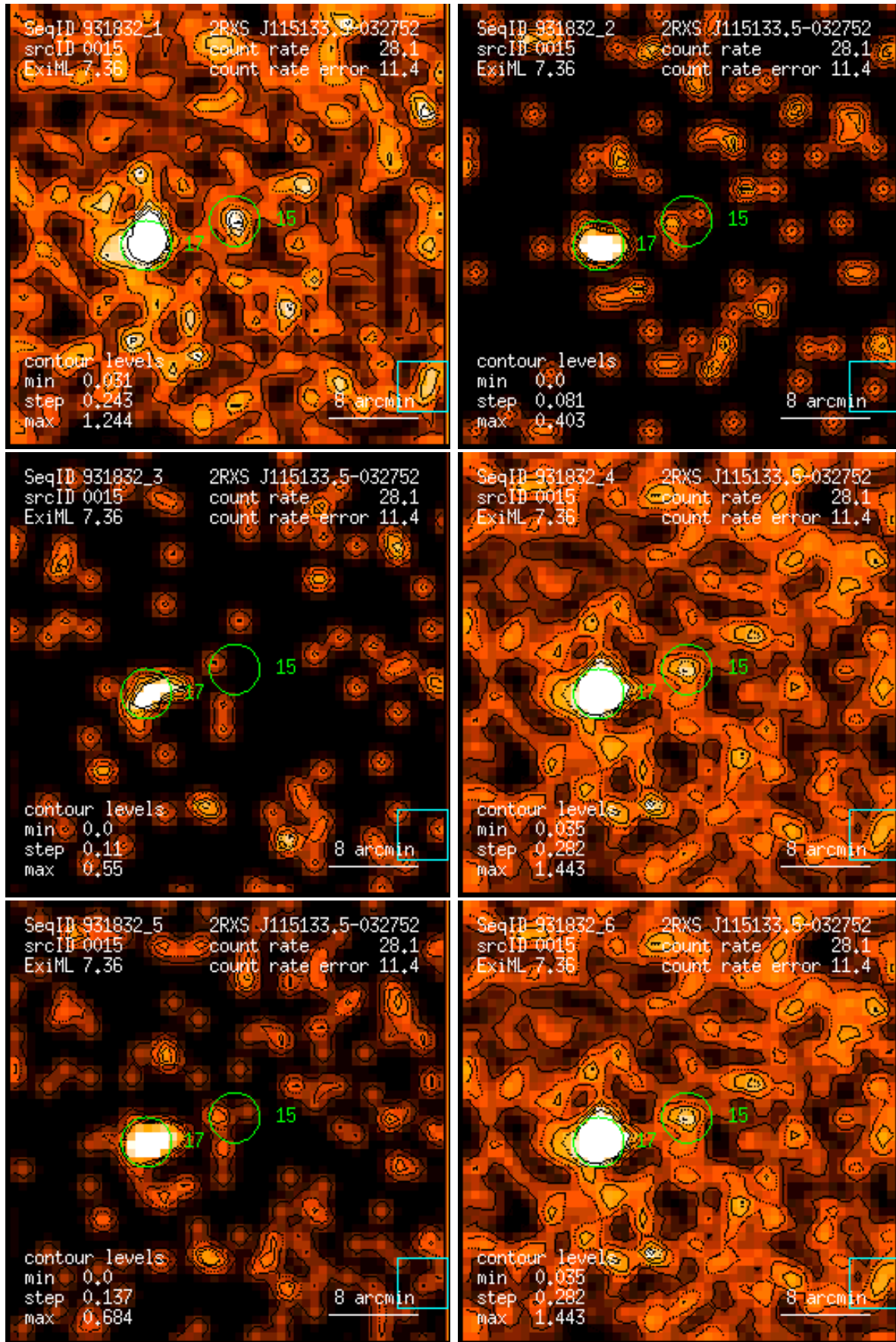
Figure 15: RASS 931832: detection 0015: band rate images, Gaussian filter: (1) PSPC channels 11 – 41, (2) 52 – 90, (3) 91 – 201, (4) 11 – 235, (5) 52 – 201, (6) 11 – 201. Broad band rates in counts/ks. Band rate contour levels in counts/ks/arcmin 2 .
