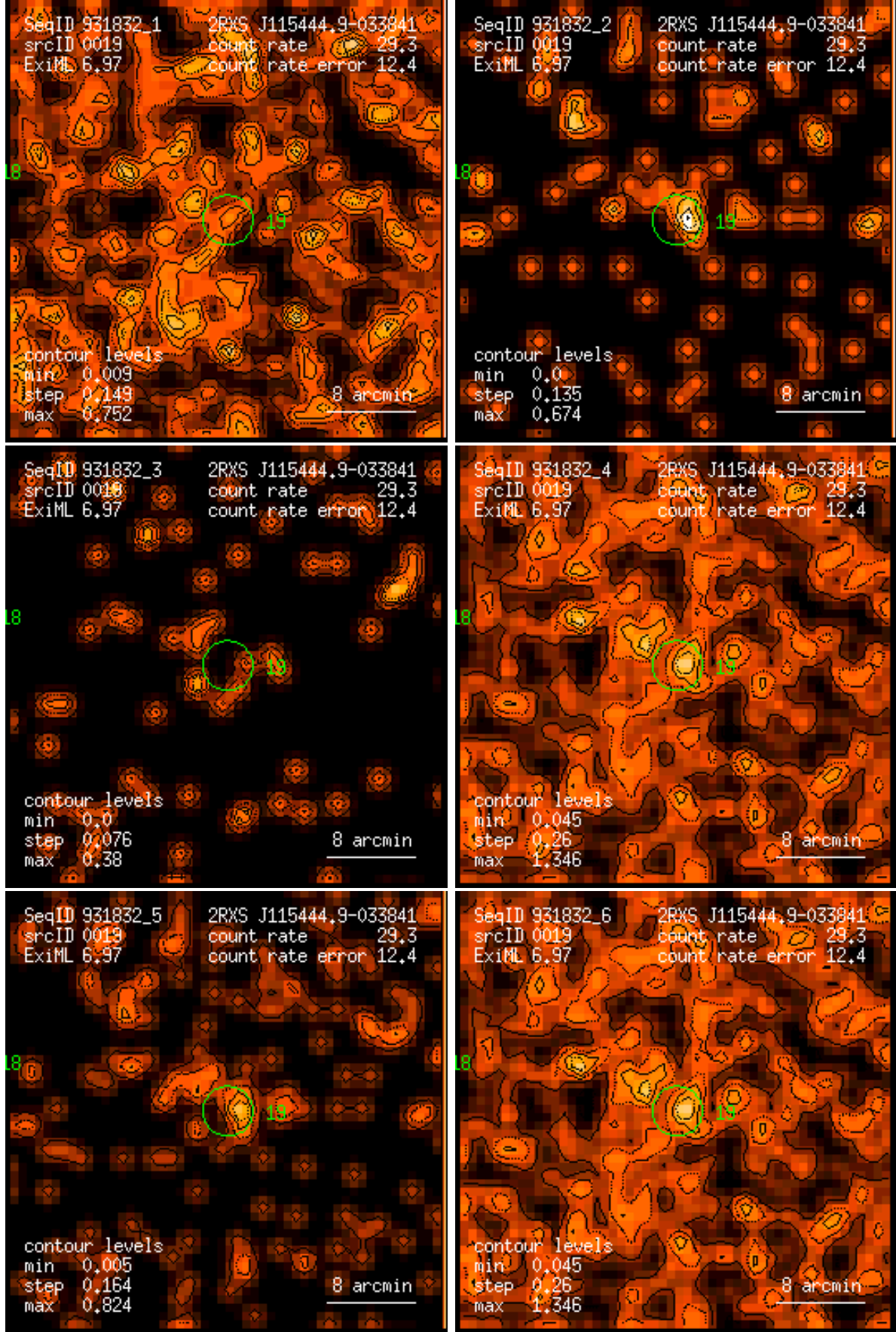
Figure 19: RASS 931832: detection 0019: band rate images, Gaussian filter: (1) PSPC channels 11 – 41, (2) 52 – 90, (3) 91 – 201, (4) 11 – 235, (5) 52 – 201, (6) 11 – 201. Broad band rates in counts/ks. Band rate contour levels in counts/ks/arcmin 2 .
