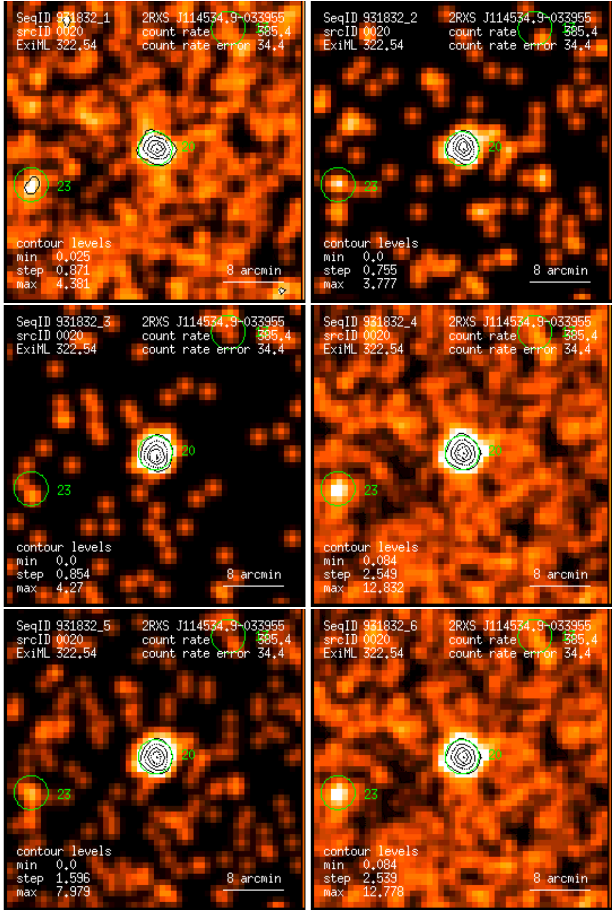
Figure 20: RASS 931832: detection 0020: band rate images, Gaussian filter: (1) PSPC channels 11 – 41, (2) 52 – 90, (3) 91 – 201, (4) 11 – 235, (5) 52 – 201, (6) 11 – 201. Broad band rates in counts/ks. Band rate contour levels in counts/ks/arcmin 2 .
