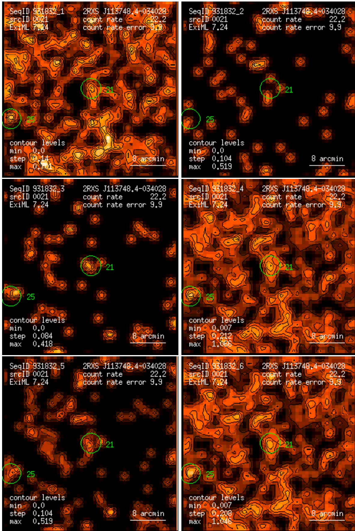
Figure 21: RASS 931832: detection 0021: band rate images, Gaussian filter: (1) PSPC channels 11 – 41, (2) 52 – 90, (3) 91 – 201, (4) 11 – 235, (5) 52 – 201, (6) 11 – 201. Broad band rates in counts/ks. Band rate contour levels in counts/ks/arcmin 2 .
