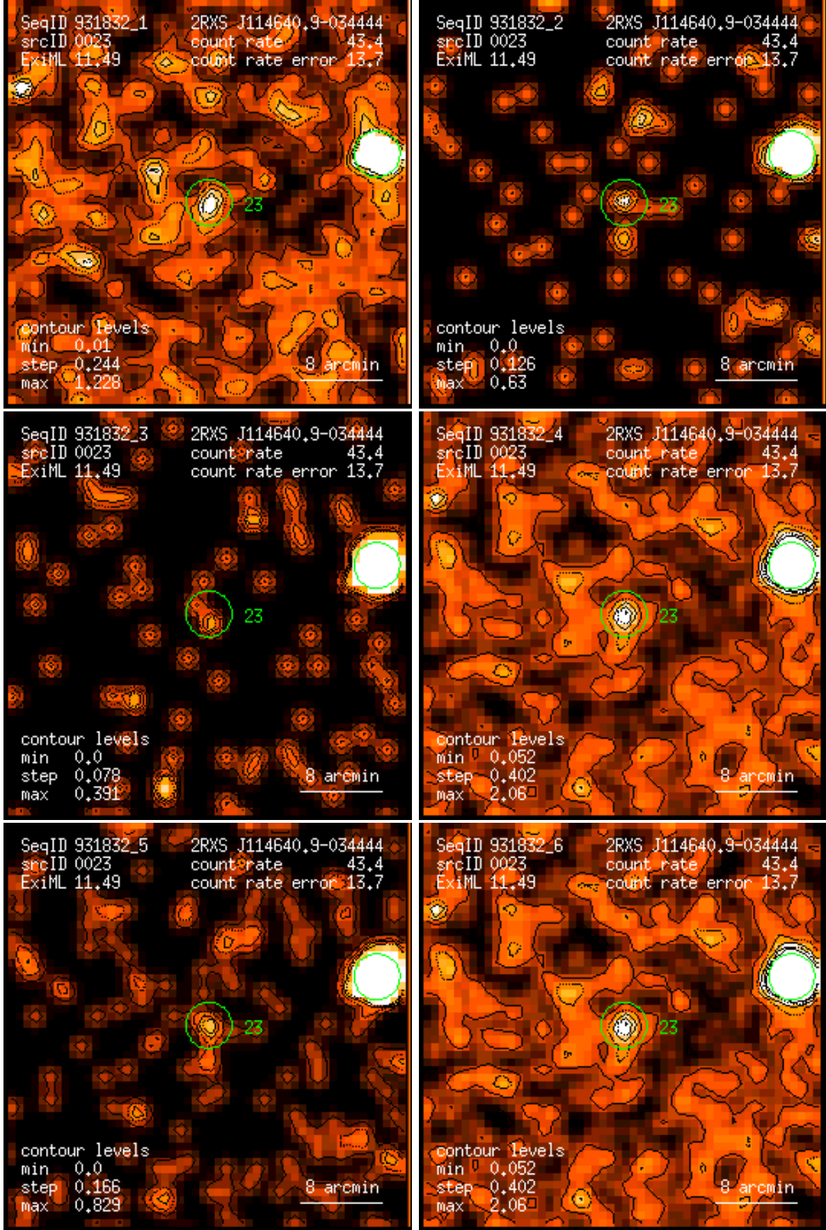
Figure 23: RASS 931832: detection 0023: band rate images, Gaussian filter: (1) PSPC channels 11 – 41, (2) 52 – 90, (3) 91 – 201, (4) 11 – 235, (5) 52 – 201, (6) 11 – 201. Broad band rates in counts/ks. Band rate contour levels in counts/ks/arcmin 2 .
