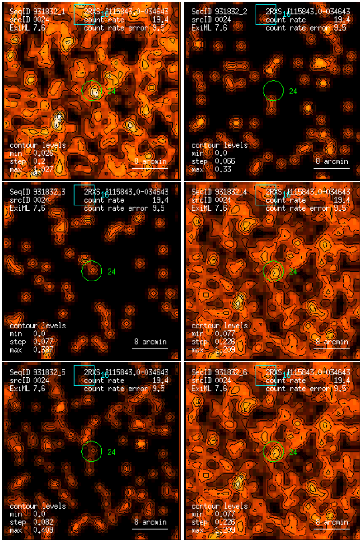
Figure 24: RASS 931832: detection 0024: band rate images, Gaussian filter: (1) PSPC channels 11 – 41, (2) 52 – 90, (3) 91 – 201, (4) 11 – 235, (5) 52 – 201, (6) 11 – 201. Broad band rates in counts/ks. Band rate contour levels in counts/ks/arcmin 2 .
