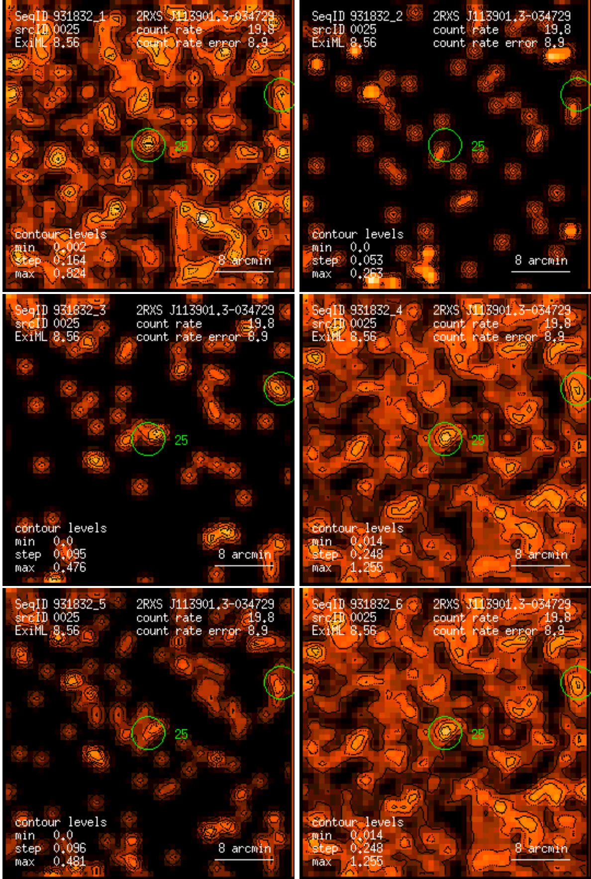
Figure 25: RASS 931832: detection 0025: band rate images, Gaussian filter: (1) PSPC channels 11 – 41, (2) 52 – 90, (3) 91 – 201, (4) 11 – 235, (5) 52 – 201, (6) 11 – 201. Broad band rates in counts/ks. Band rate contour levels in counts/ks/arcmin 2 .
