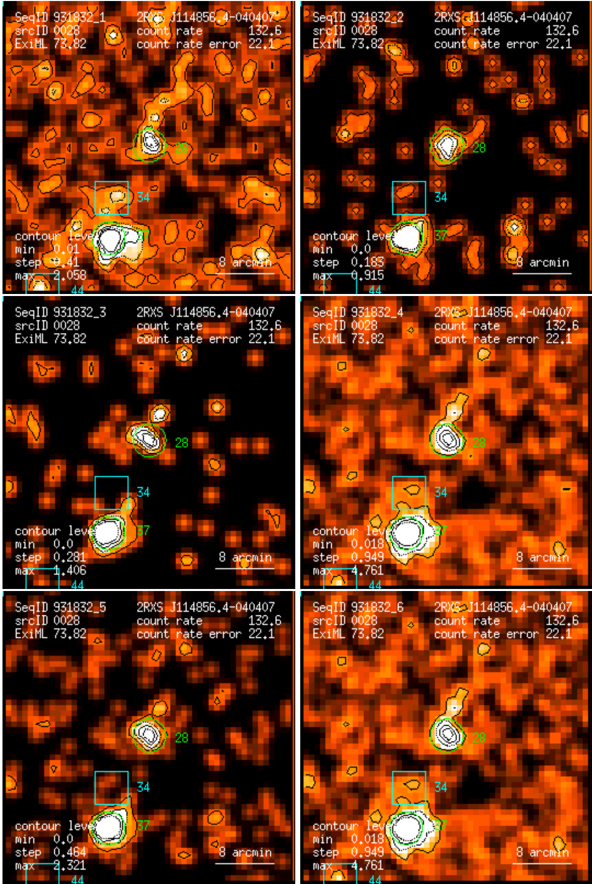
Figure 28: RASS 931832: detection 0028: band rate images, Gaussian filter: (1) PSPC channels 11 – 41, (2) 52 – 90, (3) 91 – 201, (4) 11 – 235, (5) 52 – 201, (6) 11 – 201. Broad band rates in counts/ks. Band rate contour levels in counts/ks/arcmin 2 .
