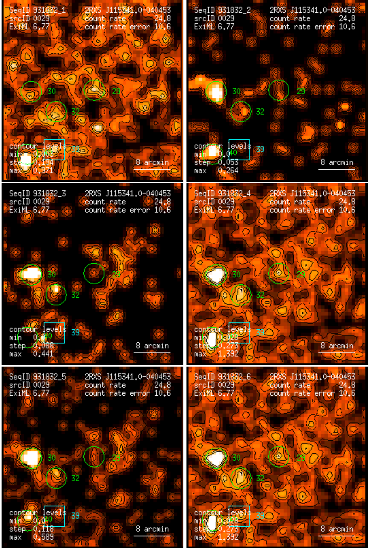
Figure 29: RASS 931832: detection 0029: band rate images, Gaussian filter: (1) PSPC channels 11 – 41, (2) 52 – 90, (3) 91 – 201, (4) 11 – 235, (5) 52 – 201, (6) 11 – 201. Broad band rates in counts/ks. Band rate contour levels in counts/ks/arcmin 2 .
