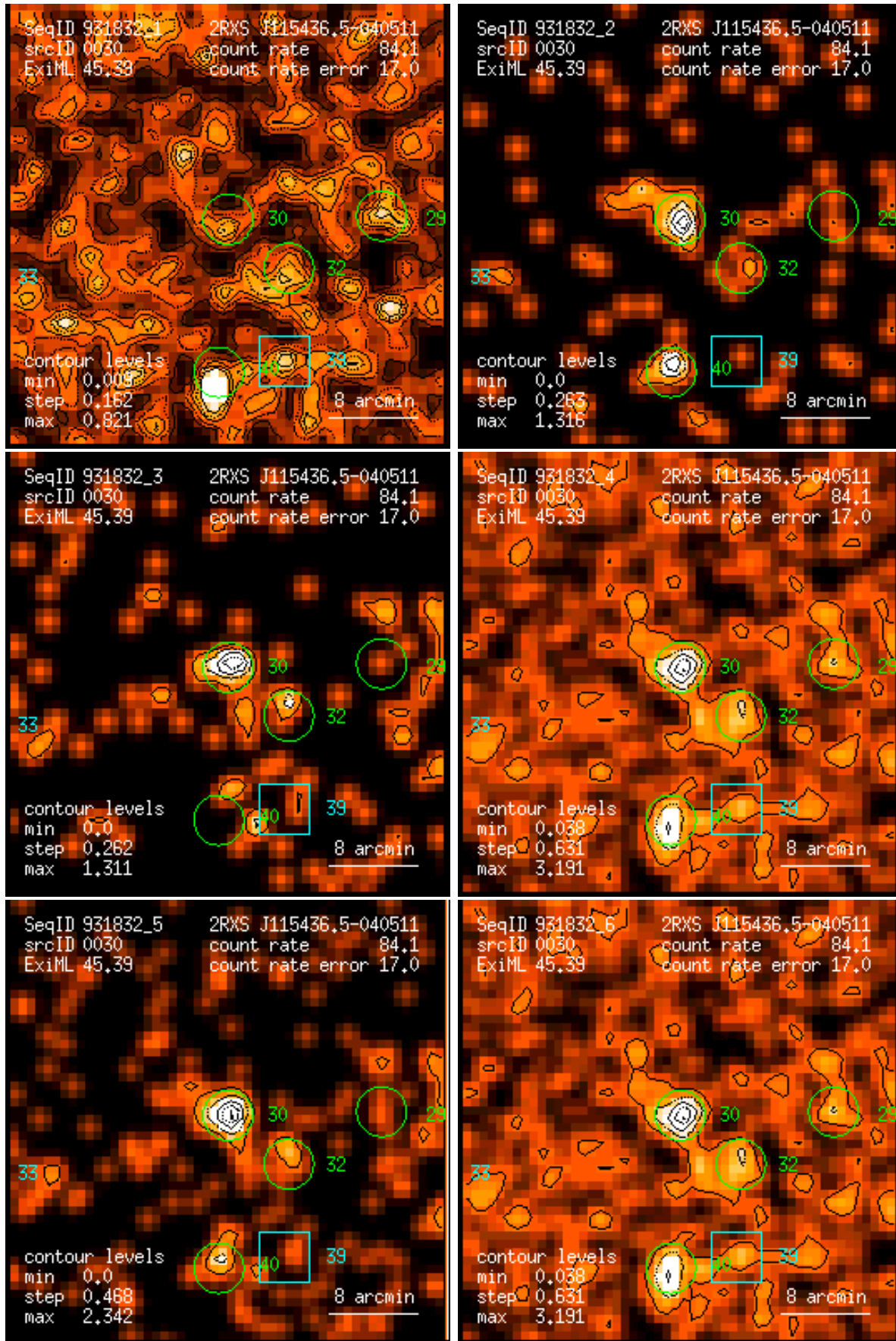
Figure 30: RASS 931832: detection 0030: band rate images, Gaussian filter: (1) PSPC channels 11 – 41, (2) 52 – 90, (3) 91 – 201, (4) 11 – 235, (5) 52 – 201, (6) 11 – 201. Broad band rates in counts/ks. Band rate contour levels in counts/ks/arcmin 2 .
