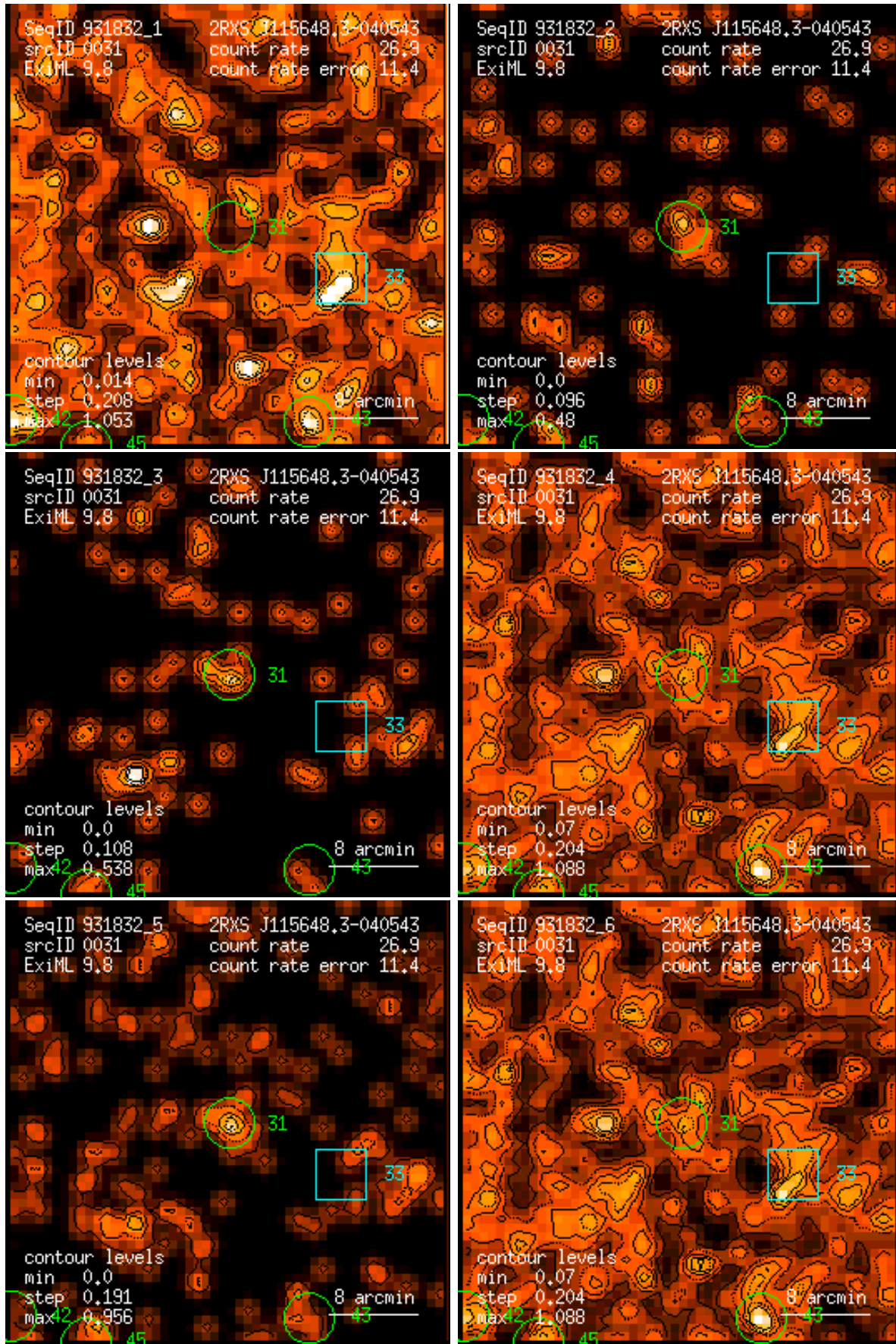
Figure 31: RASS 931832: detection 0031: band rate images, Gaussian filter: (1) PSPC channels 11 – 41, (2) 52 – 90, (3) 91 – 201, (4) 11 – 235, (5) 52 – 201, (6) 11 – 201. Broad band rates in counts/ks. Band rate contour levels in counts/ks/arcmin 2 .
