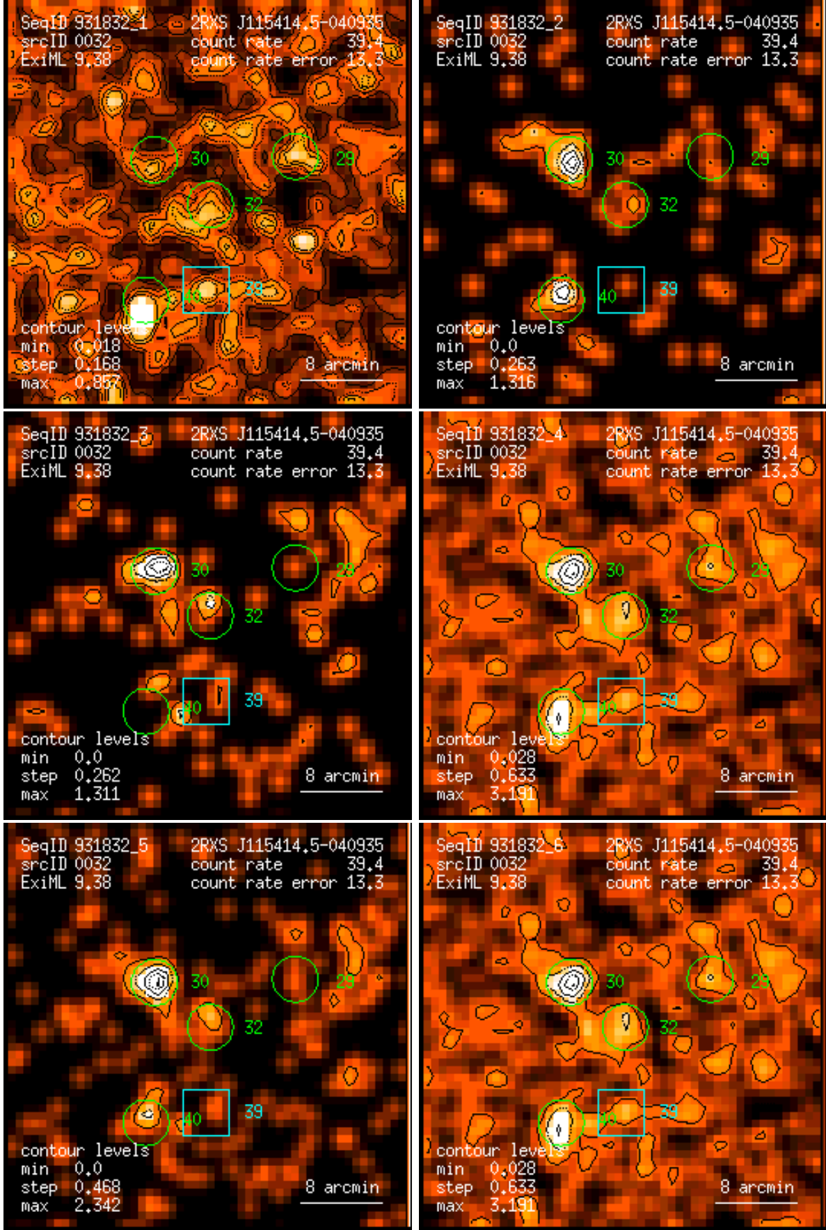
Figure 32: RASS 931832: detection 0032: band rate images, Gaussian filter: (1) PSPC channels 11 – 41, (2) 52 – 90, (3) 91 – 201, (4) 11 – 235, (5) 52 – 201, (6) 11 – 201. Broad band rates in counts/ks. Band rate contour levels in counts/ks/arcmin 2 .
